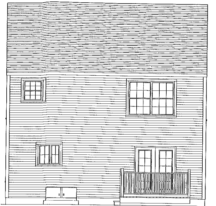
LEFT ELEVATION
