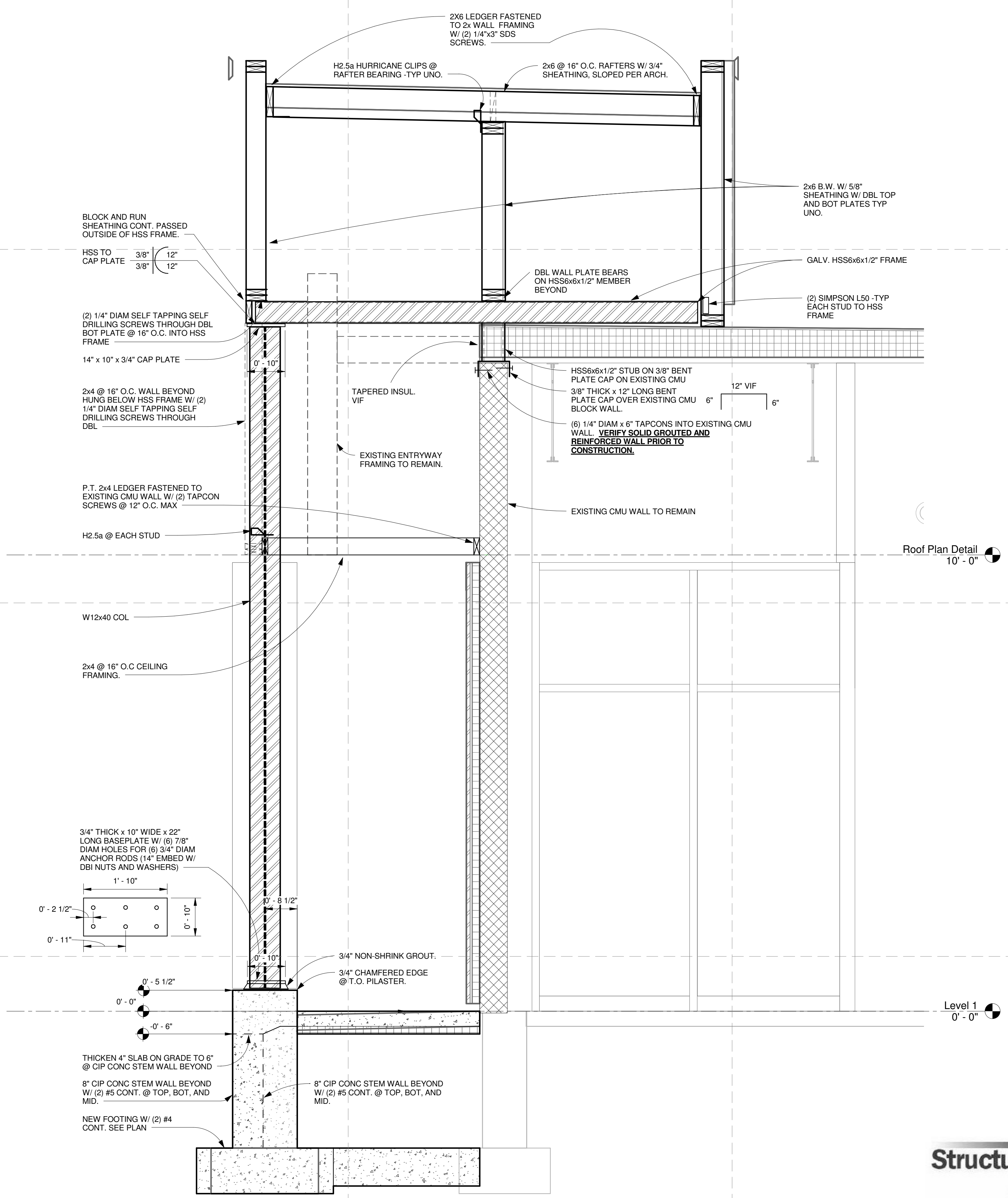
1 Section 1 3/4" = 1'-0"
