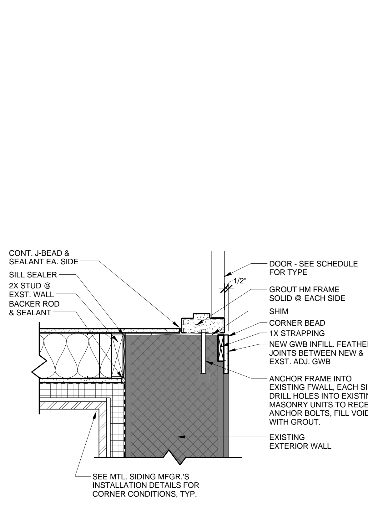
B4 PLAN DETAIL - DOOR JAMB @ ATM 1 1/2" = 1'-0"
