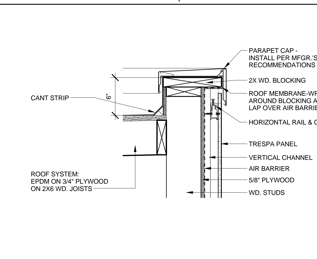
D1 DETAIL - PARAPET @ ENTRY CANOPY 1 1/2" = 1'-0"
