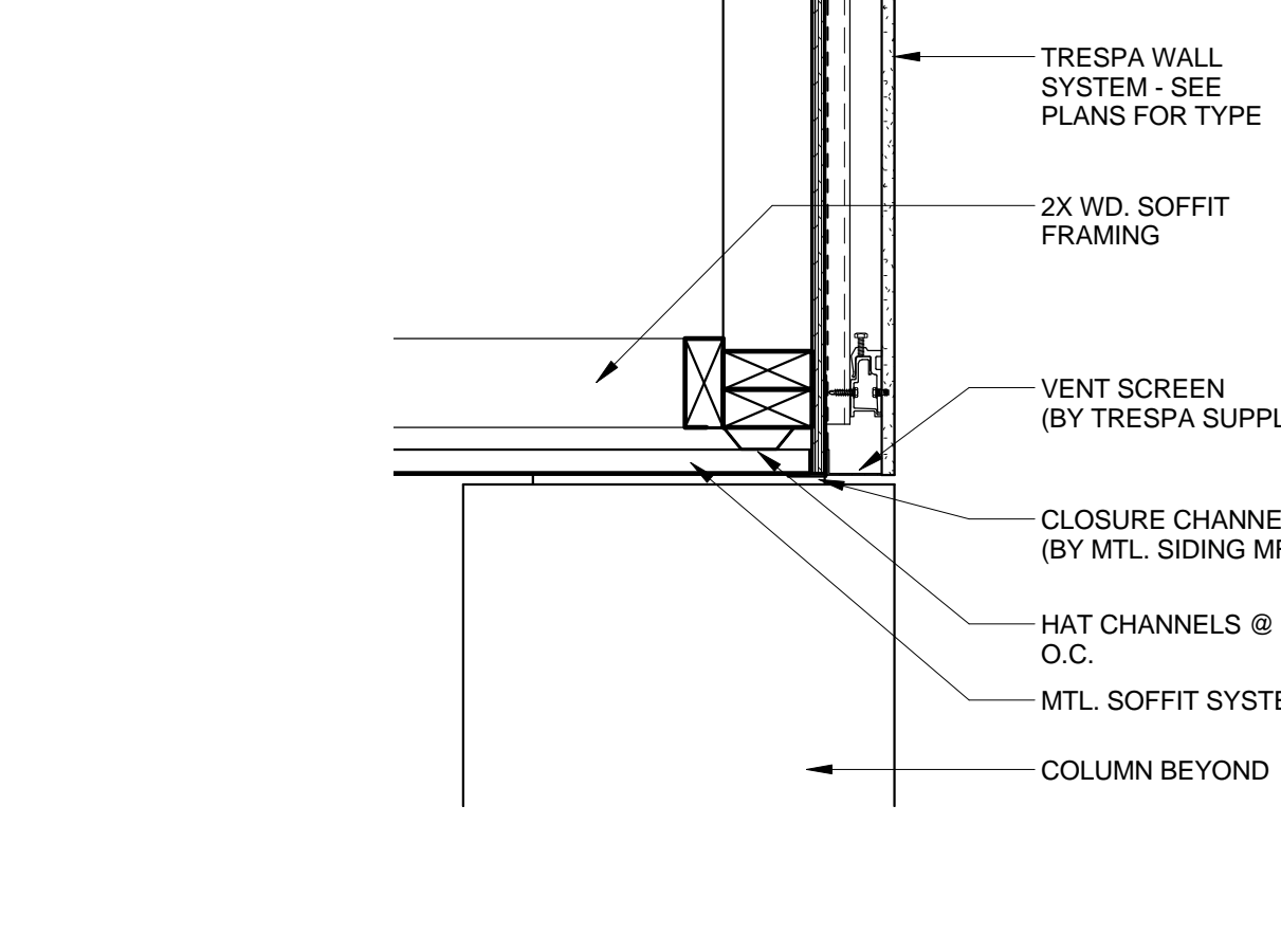
B1 DETAIL - SOFFIT @ ENTRY CANOPY 1 1/2" = 1'-0"
