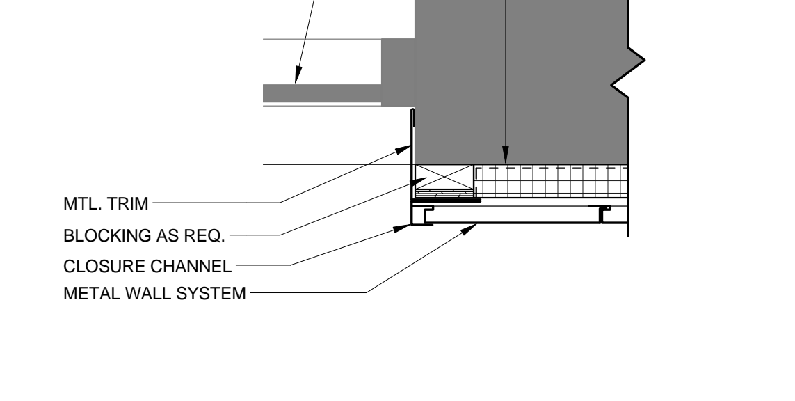
C3 DETAIL - MTL. SIDING RETURN - TYP. 1 1/2" = 1'-0"
