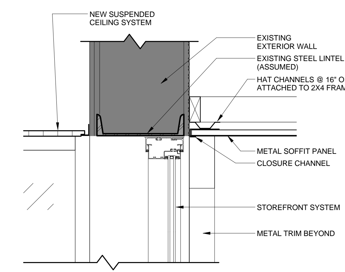
B3 SECTION DETAIL - HEAD @ EXT. STOREFRONT 1 1/2" = 1'-0"
