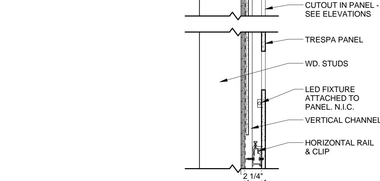
C1 DETAIL @ CANOPY CUTOUT 1 1/2" = 1'-0"
