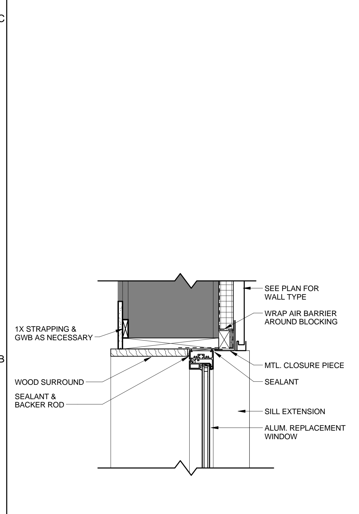
B5 JAMB @ REPLACEMENT WINDOW 1 1/2" = 1'-0"
