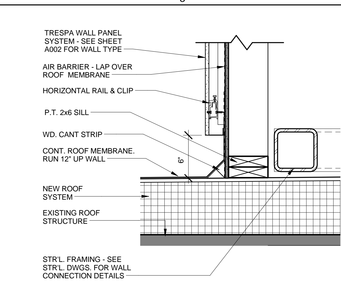
D3 DETAIL - NEW CANOPY WALL ON EXST. ROOF 1 1/2" = 1'-0"
