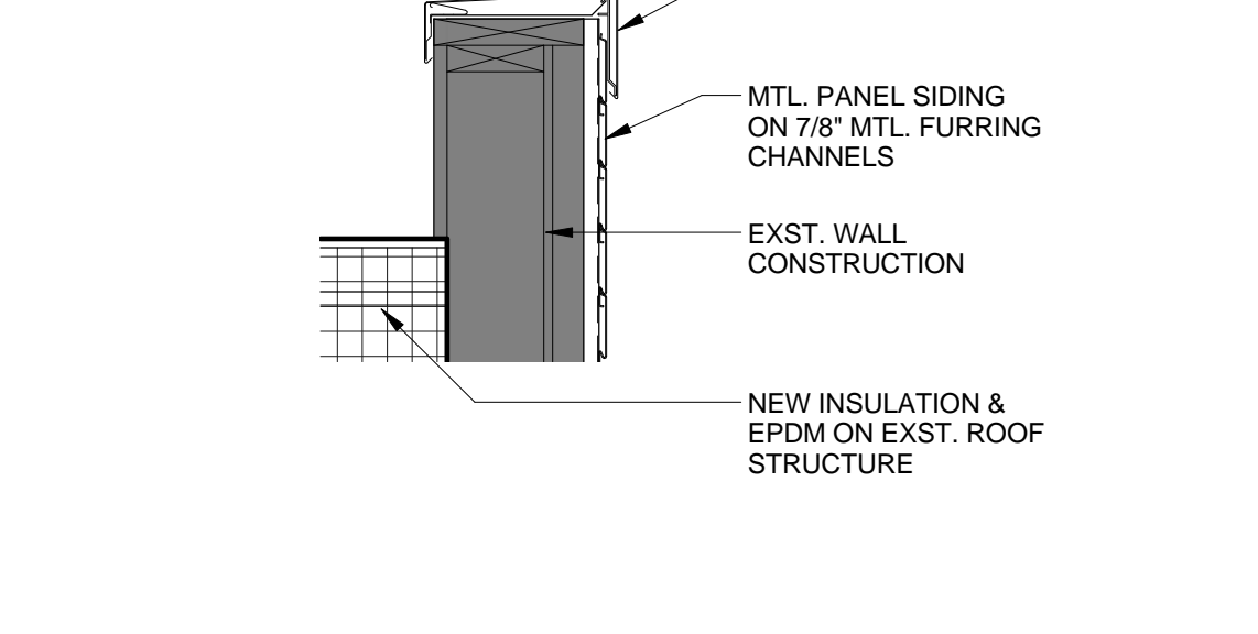
C2 PARAPET @ EXISTING CANOPY 1" = 1'-0"
