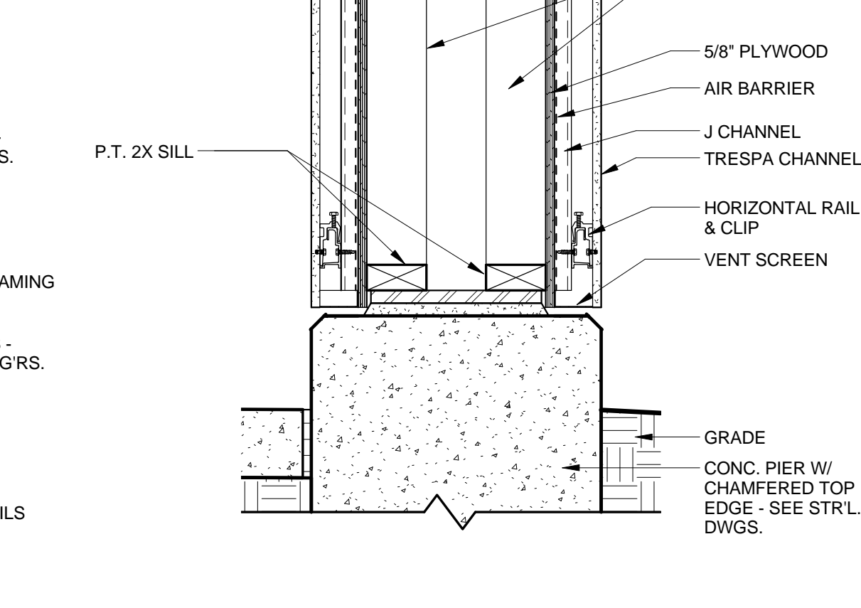
A1 SECTION - COLUMN @ ENTRY 1 1/2" = 1'-0"
