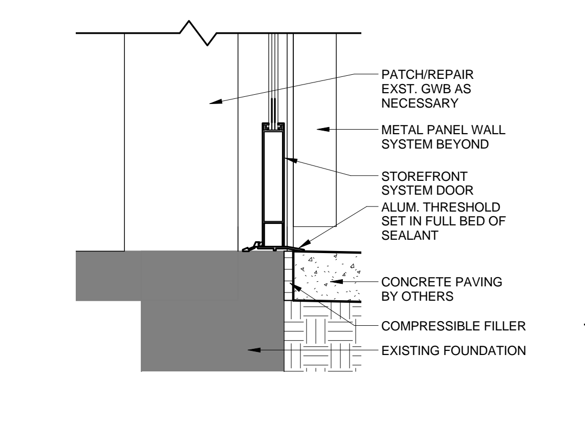
A3 DETAIL - SILL @ EXT. STOREFRONT ENTRY 1 1/2" = 1'-0"
