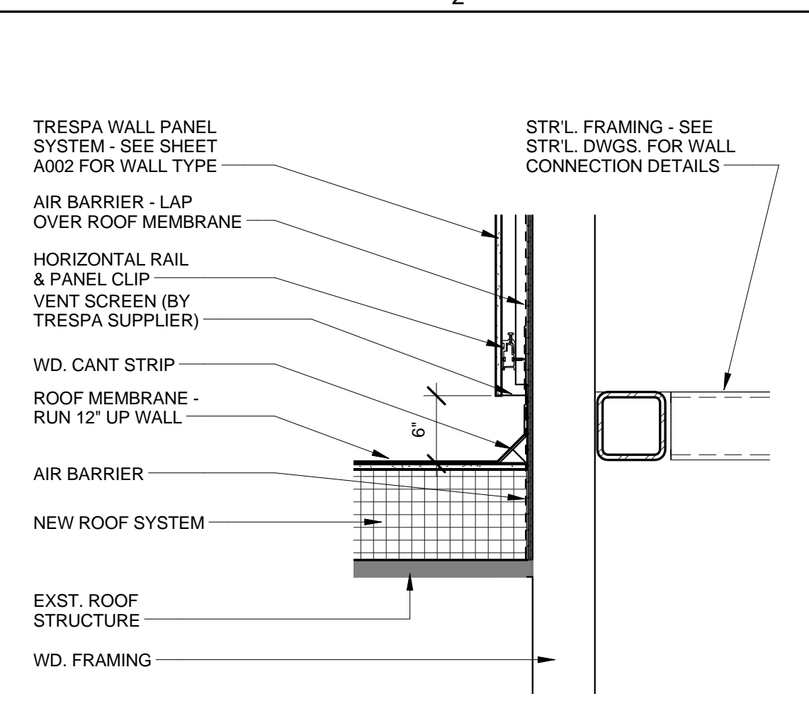
D2 CANOPY WALL - ROOF INTERSECTION 1" = 1'-0"
