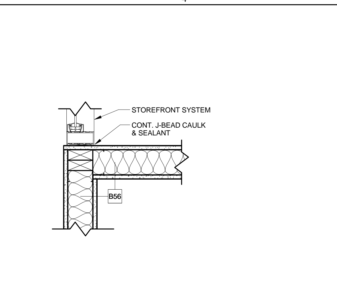
D4 PLAN DETAIL @ WALL CONNECT 1 1/2" = 1'-0"
