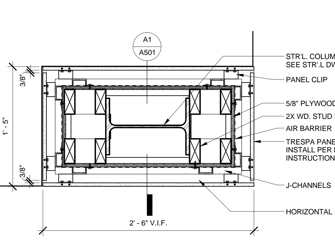
A2 PLAN DETAIL - COLUMN @ ENTRY 1 1/2" = 1'-0"
