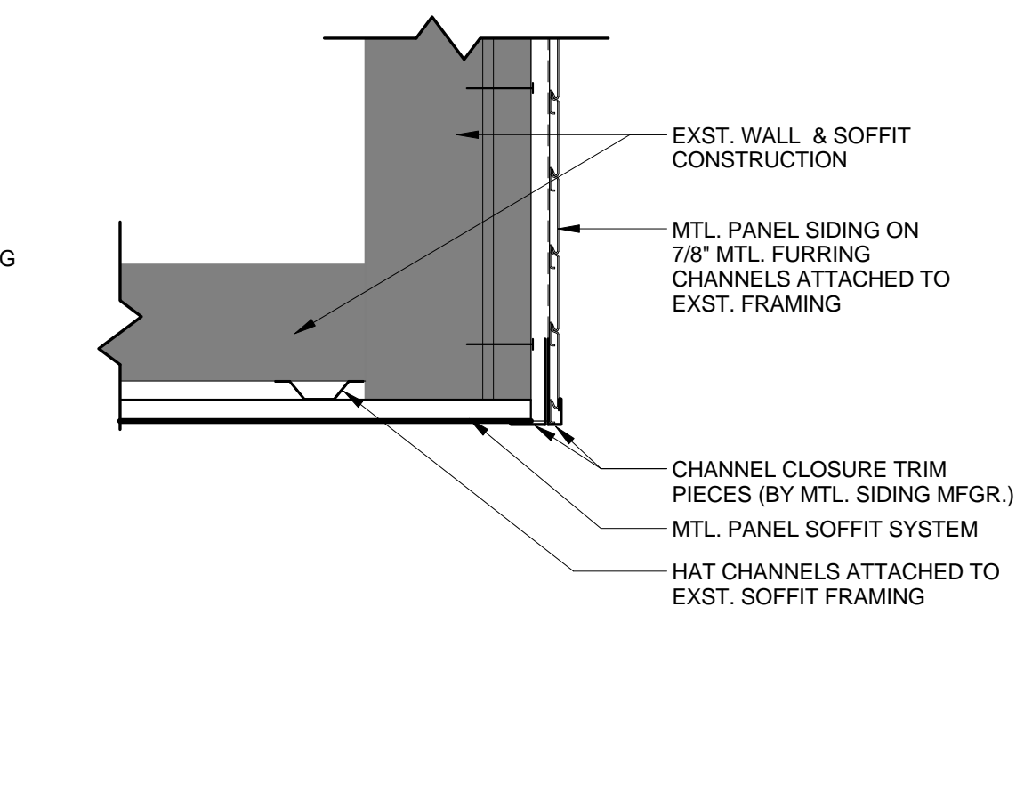
B2 NEW SOFFIT @ EXISTING CANOPY 1 1/2" = 1'-0"
