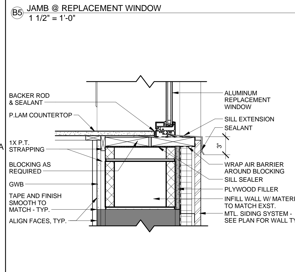
A5 DETAIL - REPLACEMENT WINDOW SILL 1 1/2" = 1'-0"
