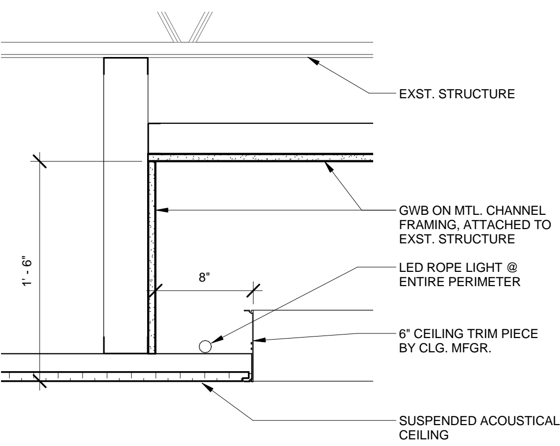
B5 DETAIL @ OVAL CEILING 1 1/2" = 1'-0"
