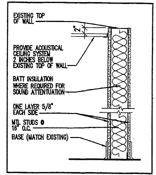
3 WALL TYPE NOT TO SCALE
