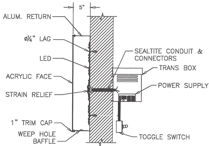
SECTION VIEW EQUIPMENT GROUNDED
