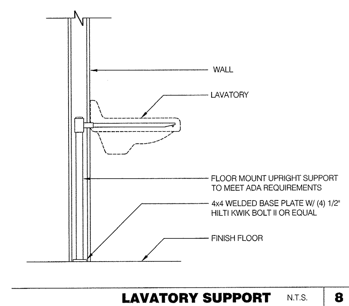
LAVATORY SUPPORT N.T.S. 8
