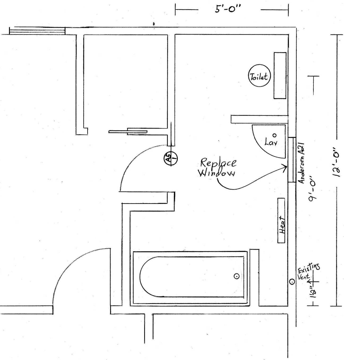
A3 - Floor Plan 47 Summit Street Proposed Master Bathroom Michael & Linda Huitt Scale: 1/2" = 1'-0"
