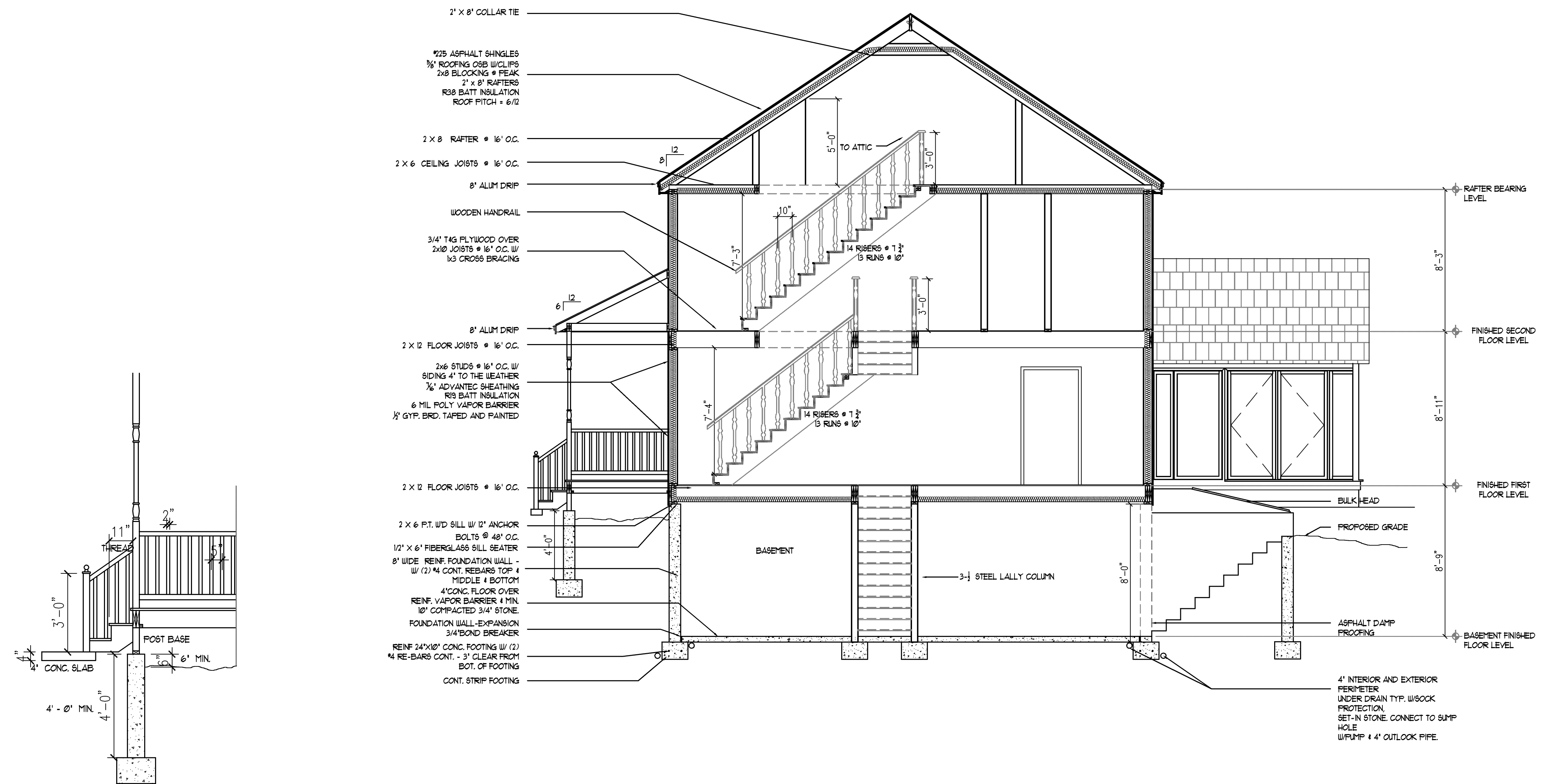
2 STAIR DETAIL 3/8" = 1'-0"
