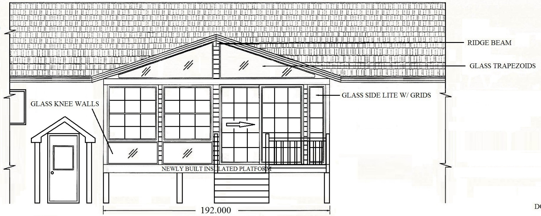
B-WALL ELEVATION
