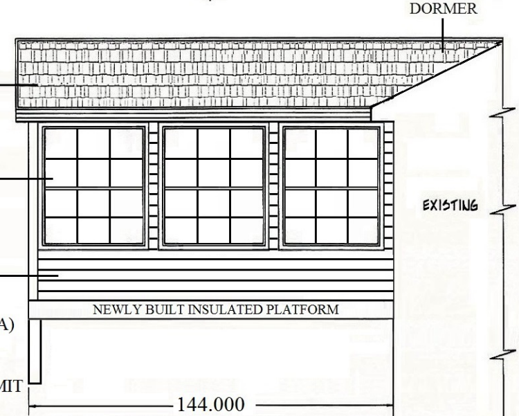
C-WALL ELEVATION
