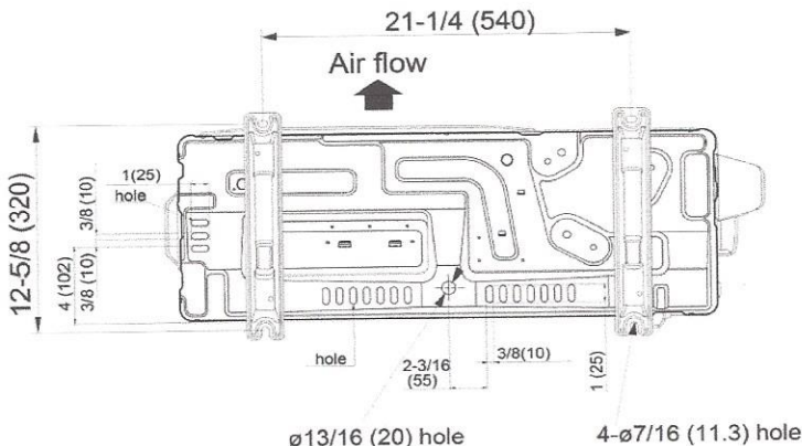
Bottom view
