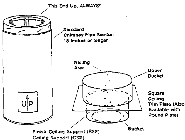
NOTE: SIZES 12" AND 14" HAVE SQUARE UPPER BUCKET FIG. 1. CEILING SUPPORT
