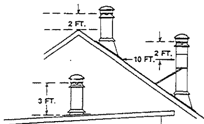
FIG. 4 RULES FOR CHIMNEY HEIGHT ABOVE THE ROOF
