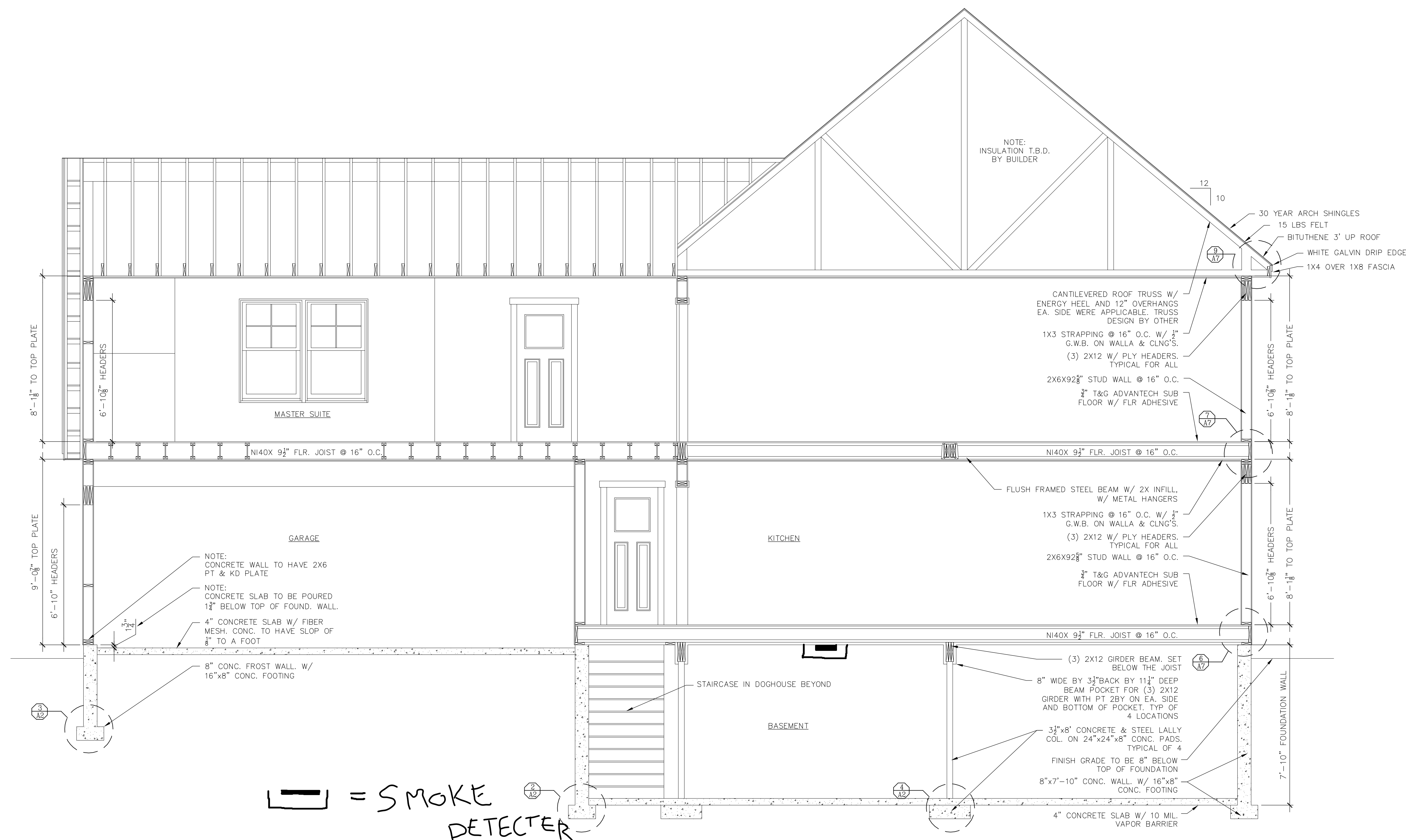
1 HOUSE & GARAGE SECTION 3/8" = 1'-0"
