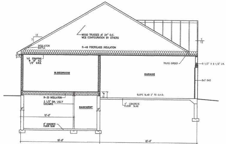
3 SECTION THRU HOUSE SCALE: 1/4" = 1' - 0"
