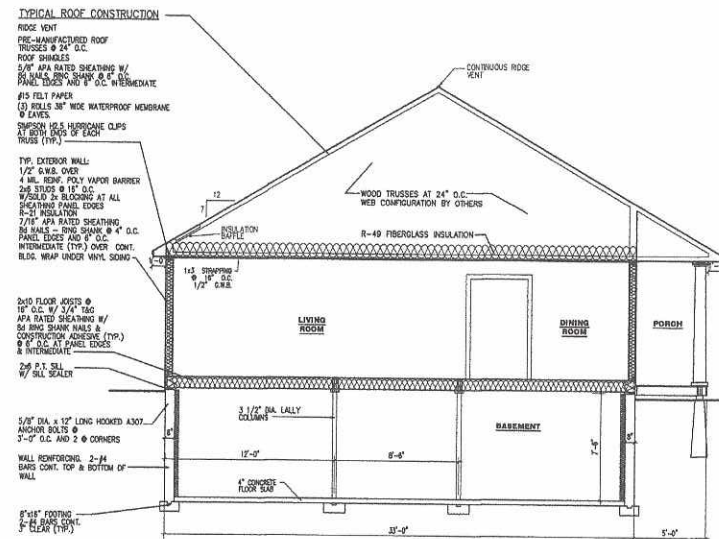
1 SECTION THRU HOUSE SCALE: 1/4" = 1' - 0"
