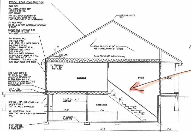
2 SECTION THRU HOUSE SCALE: 1/4" = 1' - 0"
