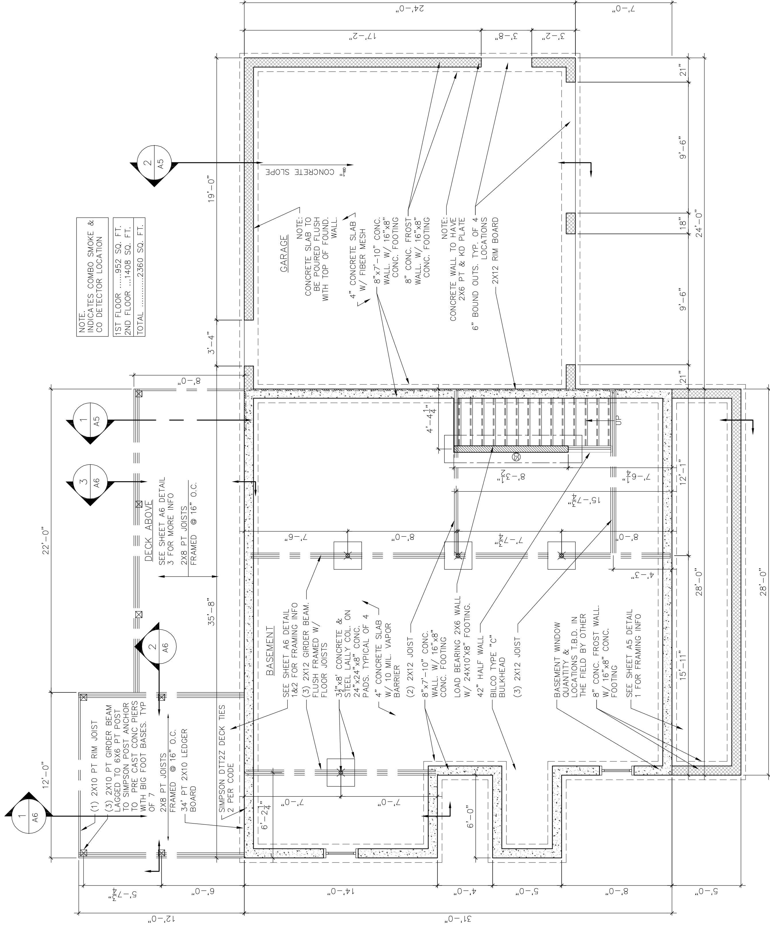
1 FOUNDATION PLAN 1/4" = 1'-0"
