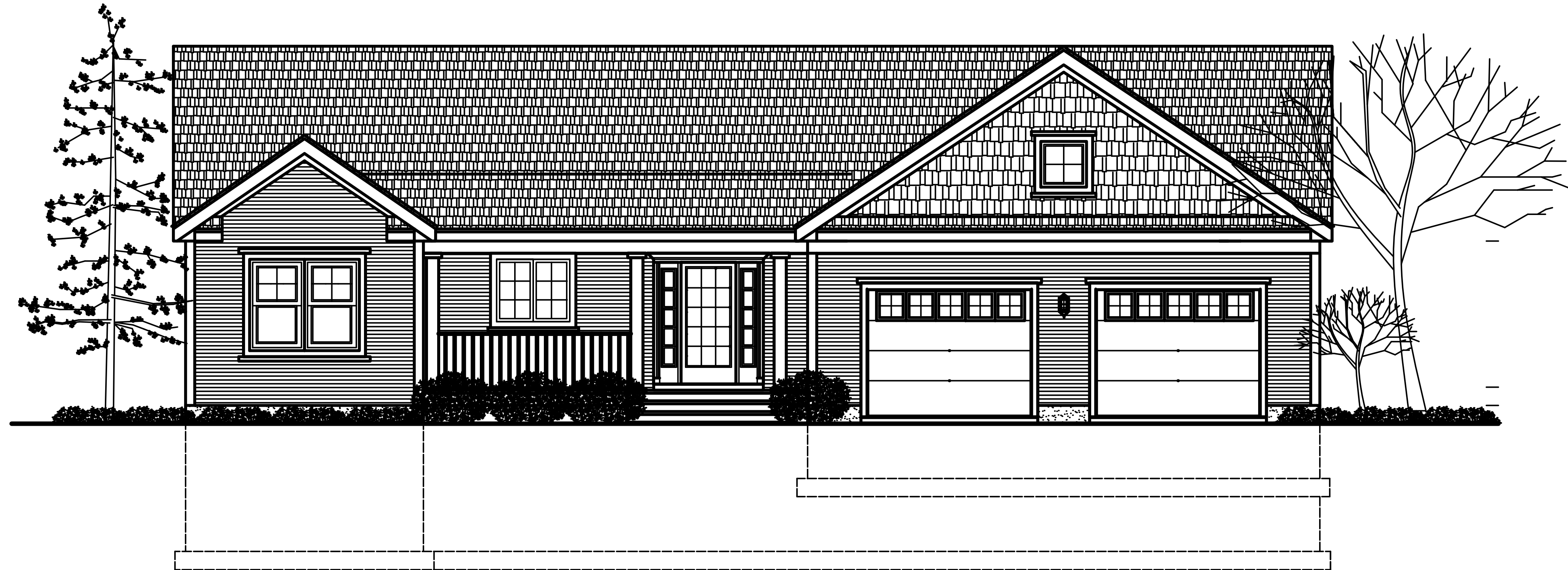
FRONT ELEVATION 1/4" = 1'-0"
