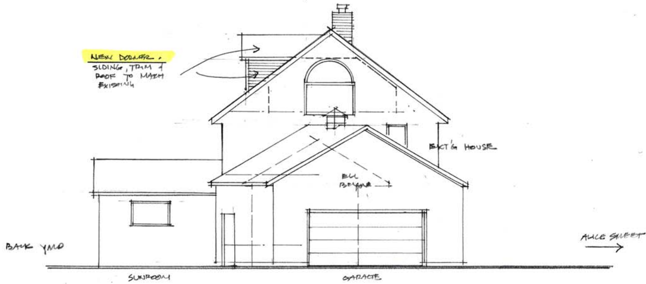
NORTH WEST ELEVATION 1/8" = 1'-0" 12.21.2013
