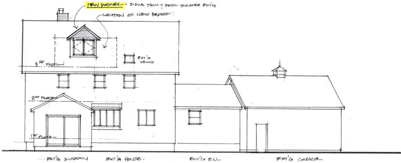
NORTH EAST (BACK) ELEVATION 1/8" = 1'-0" 12.21.2013
