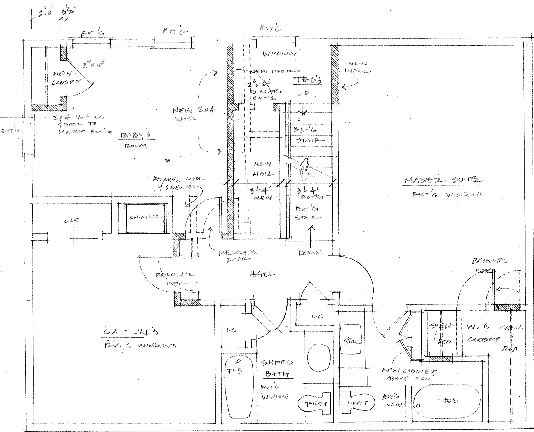
PROPOSED SECOND FLOOR PLAN 1/4" = 1'-0"
