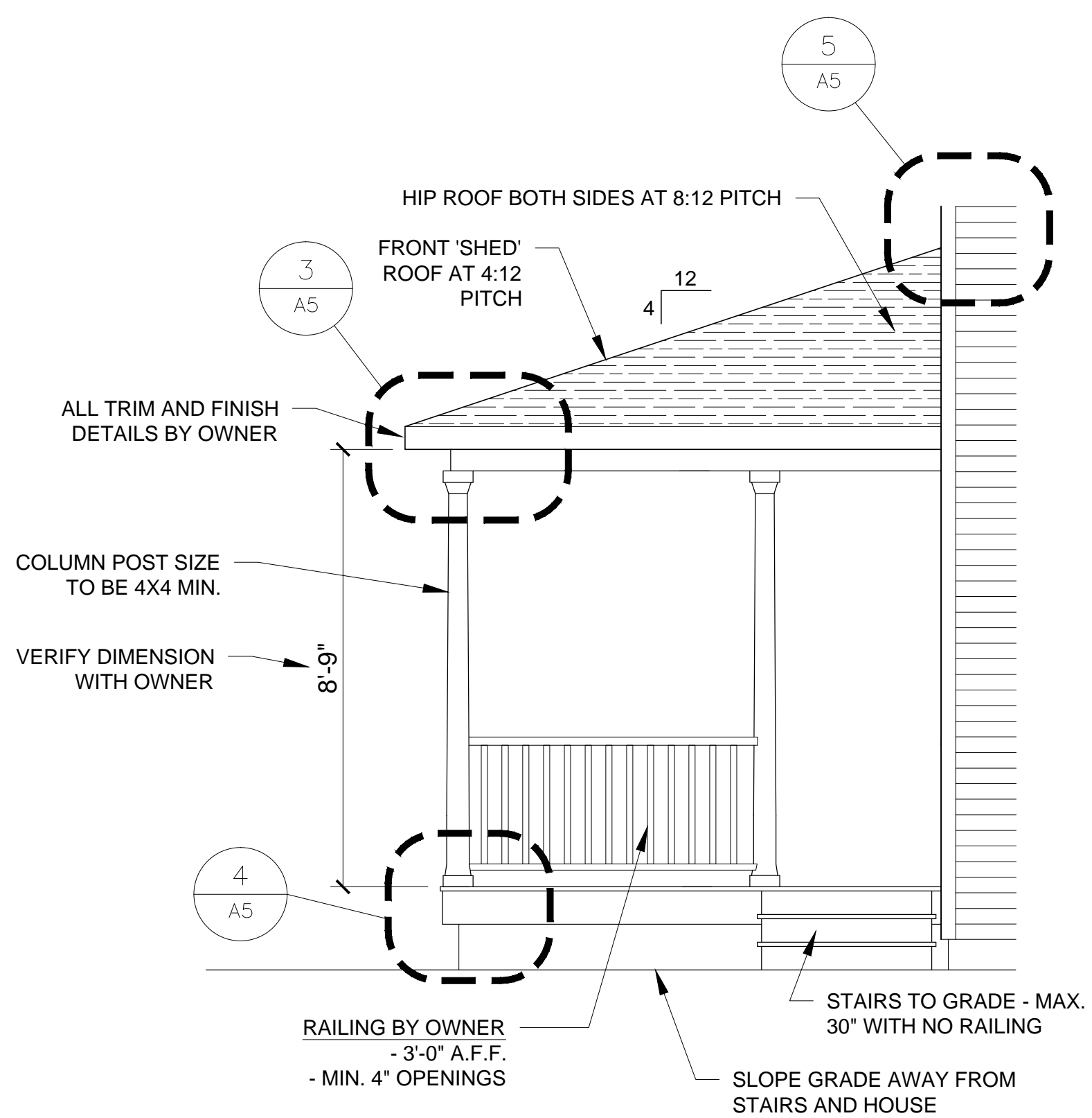
3 SIDE PORCH ELEVATION 3/8" = 1'-0" (WHEN PRINTED AT 24"X36")
