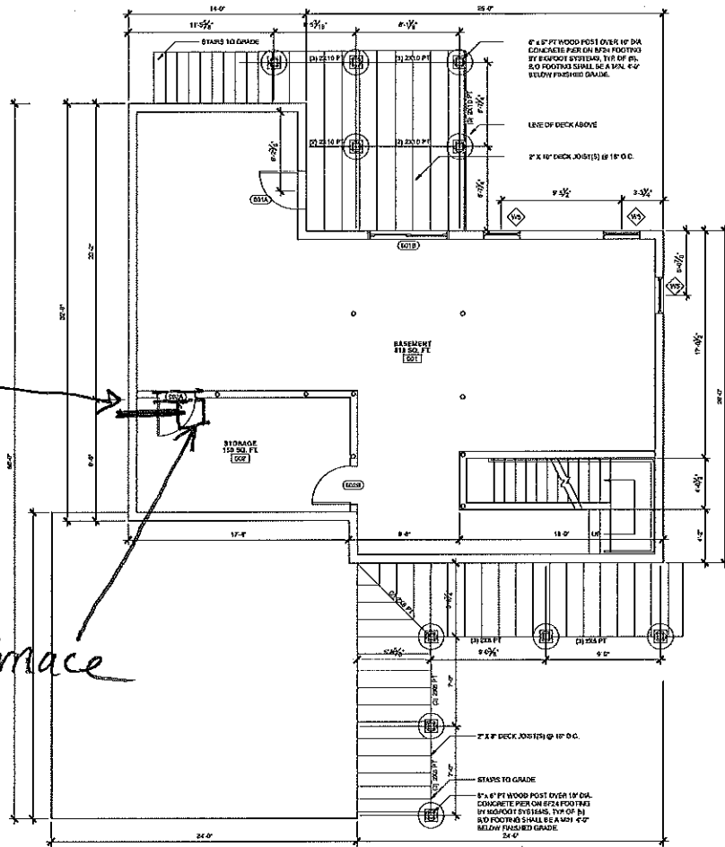
1 BASEMENT FLOOR PLAN SCALE: 1/4" = 1'-0"
