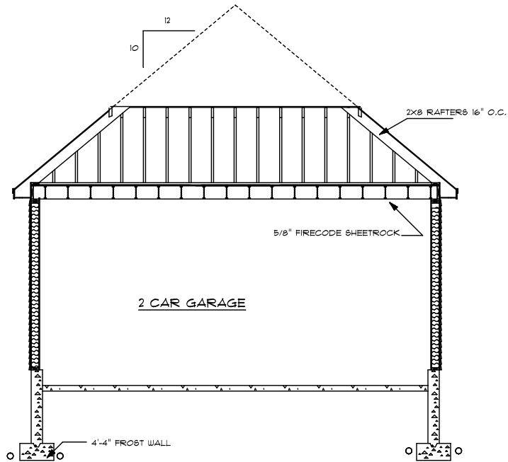
CROSS SECTION C-C SCALE: 1/4" = 1'-0"
