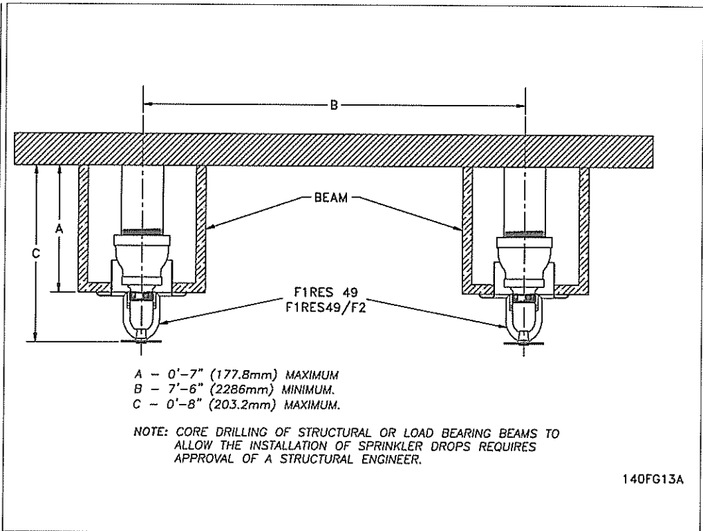
Figure 13 Pendant sprinkler positioning for beamed ceiling.
