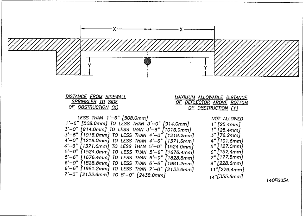
Figure 5 Positioning of sidewall sprinklers to avoid obstructions along the wall.
