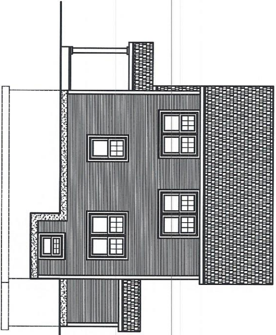
RIGHT ELEVATION V. 2.1.16
