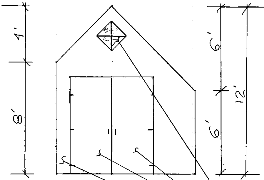
ELEVATION SIDE-WEST
