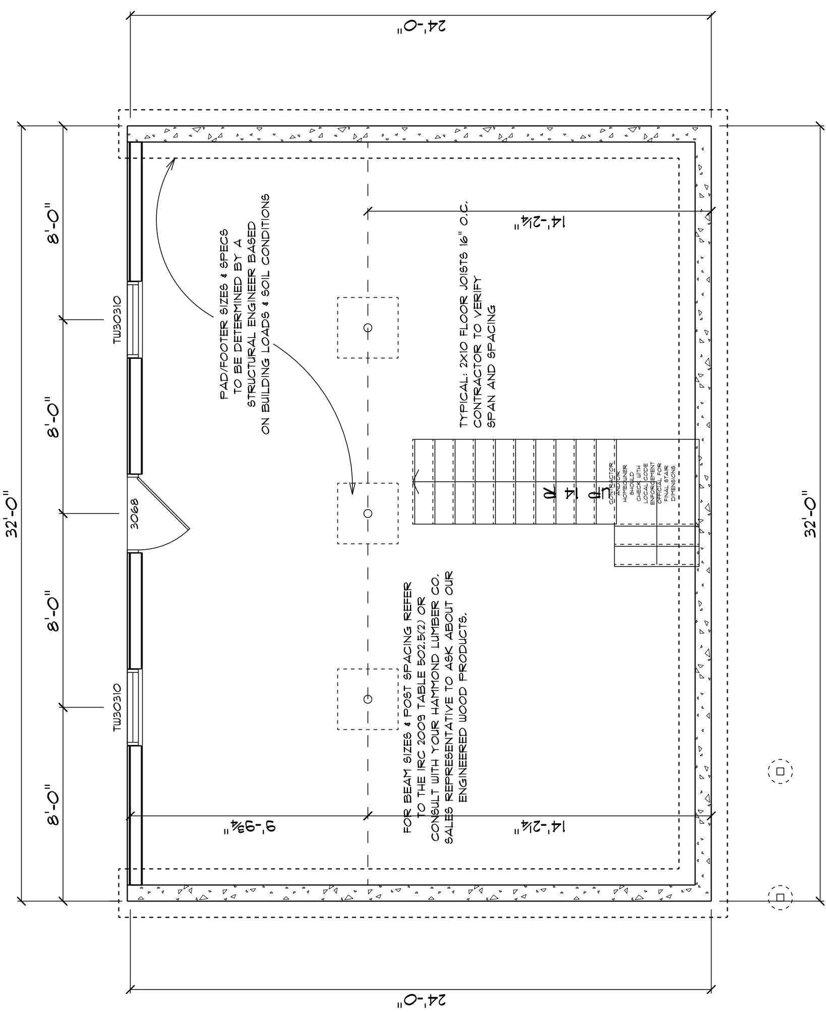
FOUNDATION SCALE: 1/4" = 1'-0"
