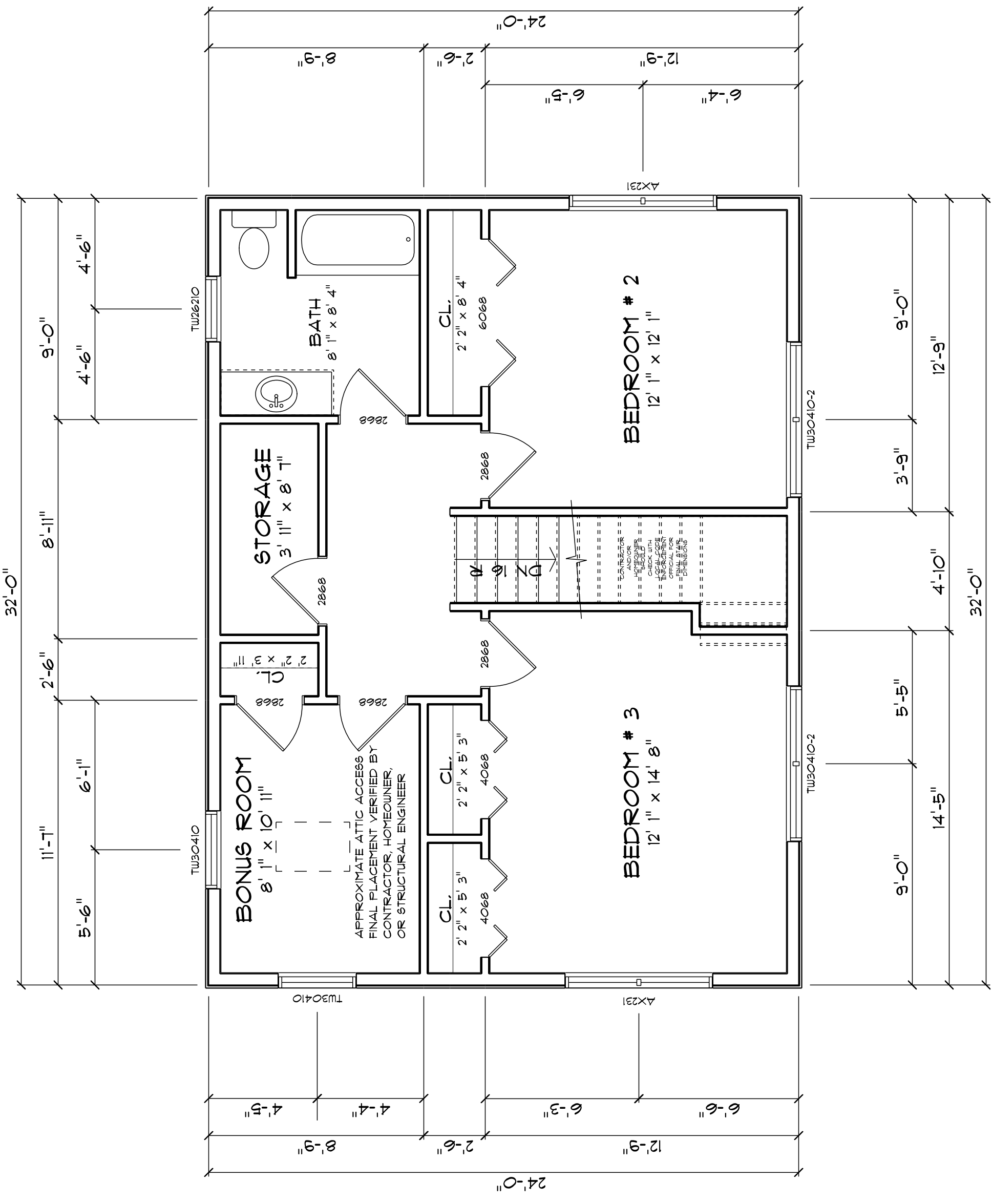
SECOND FLOOR SCALE: 1/4" = 1'-0"
