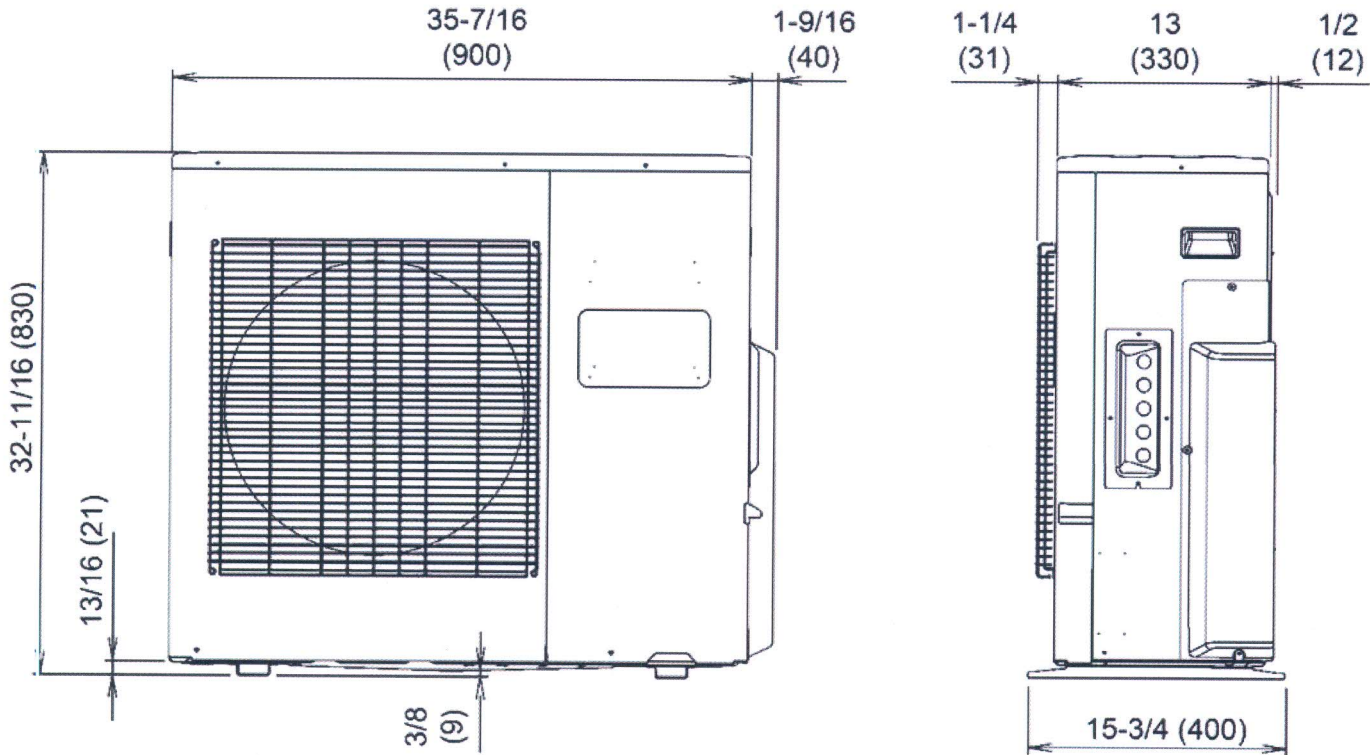
Front view
