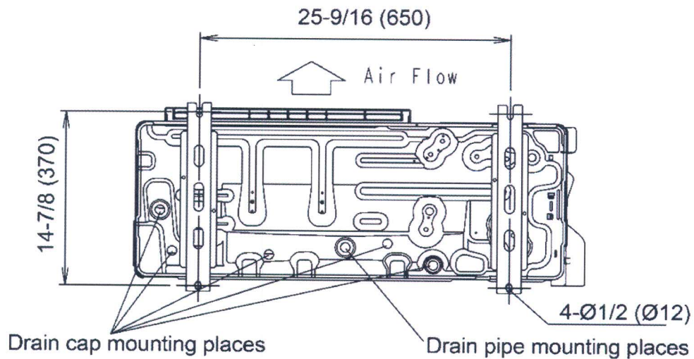
Bottom view
