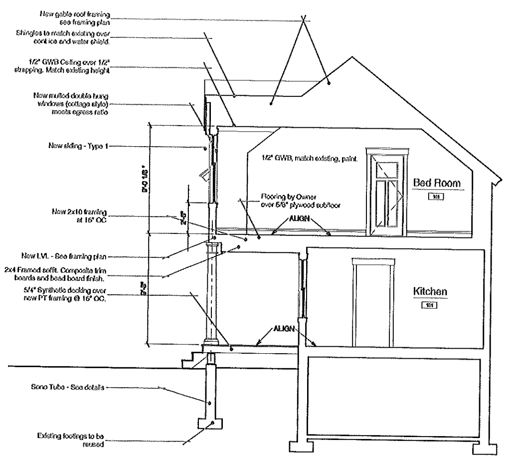
10 Proposed Section
