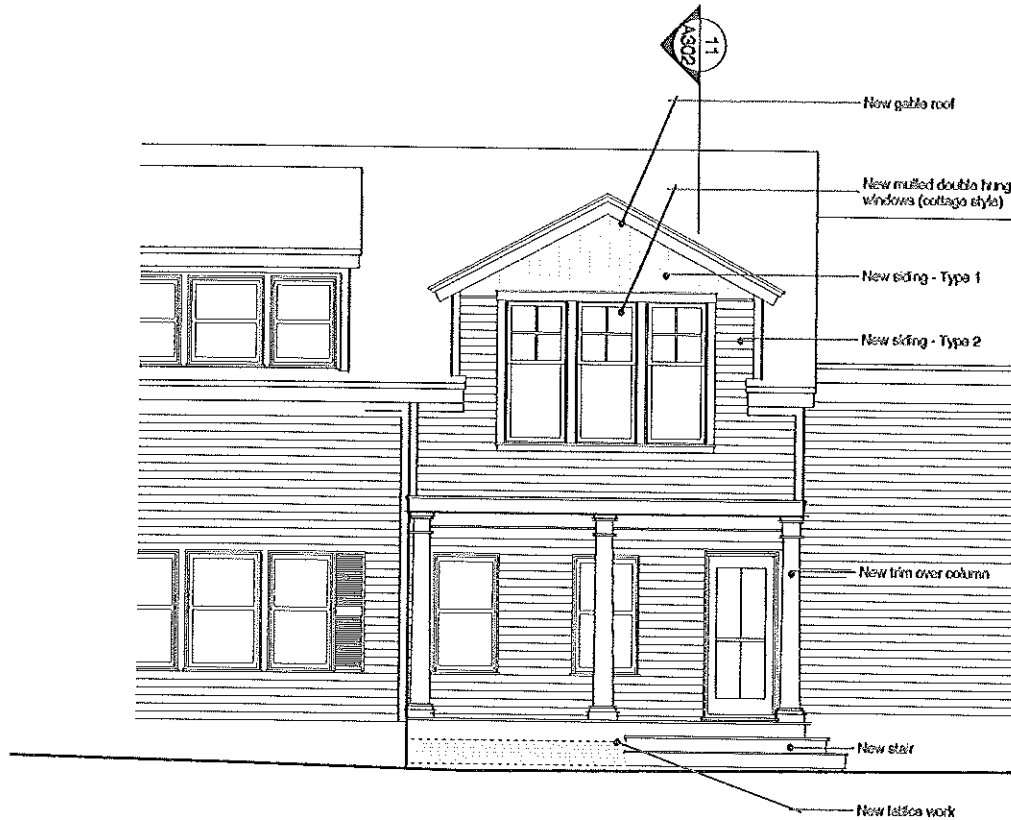
10 Proposed Elevation
