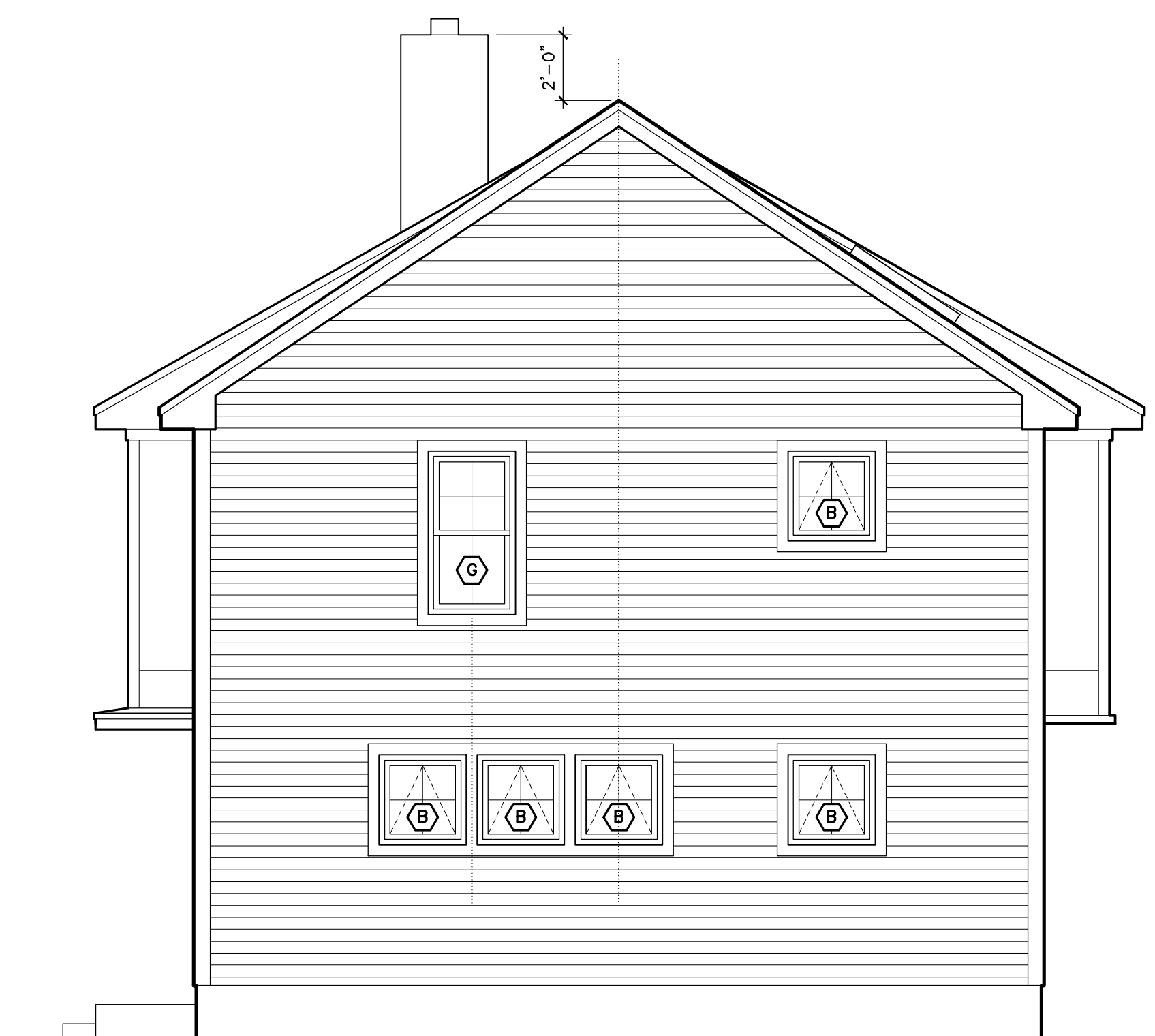
03 WEST ELEVATION (SIDE) scale: 1/4"= 1'-0"
