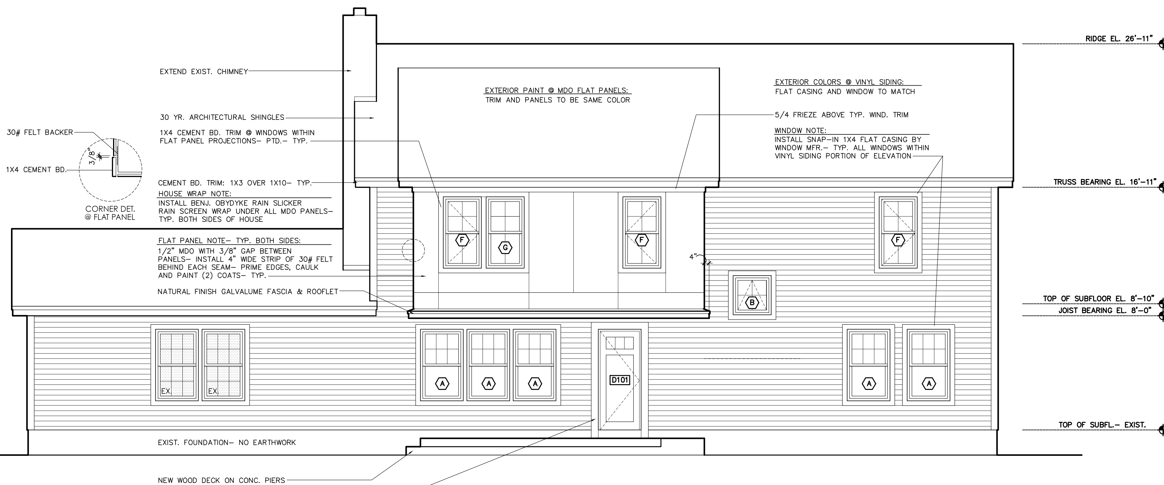
02 NORTH ELEVATION (FRONT) scale: 1/4"= 1'-0"
