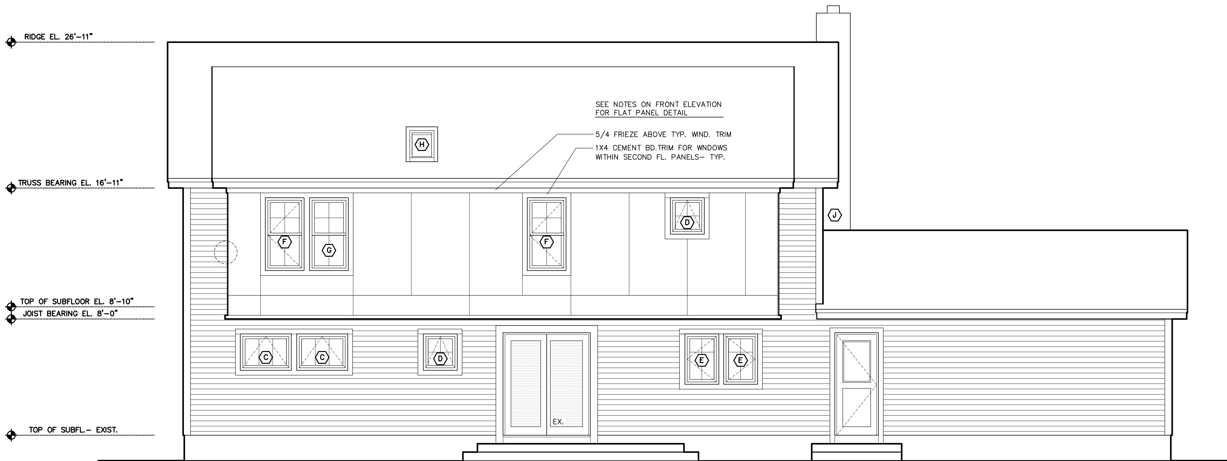
01 SOUTH ELEVATION (REAR) scale: 1/4"= 1'-0"
