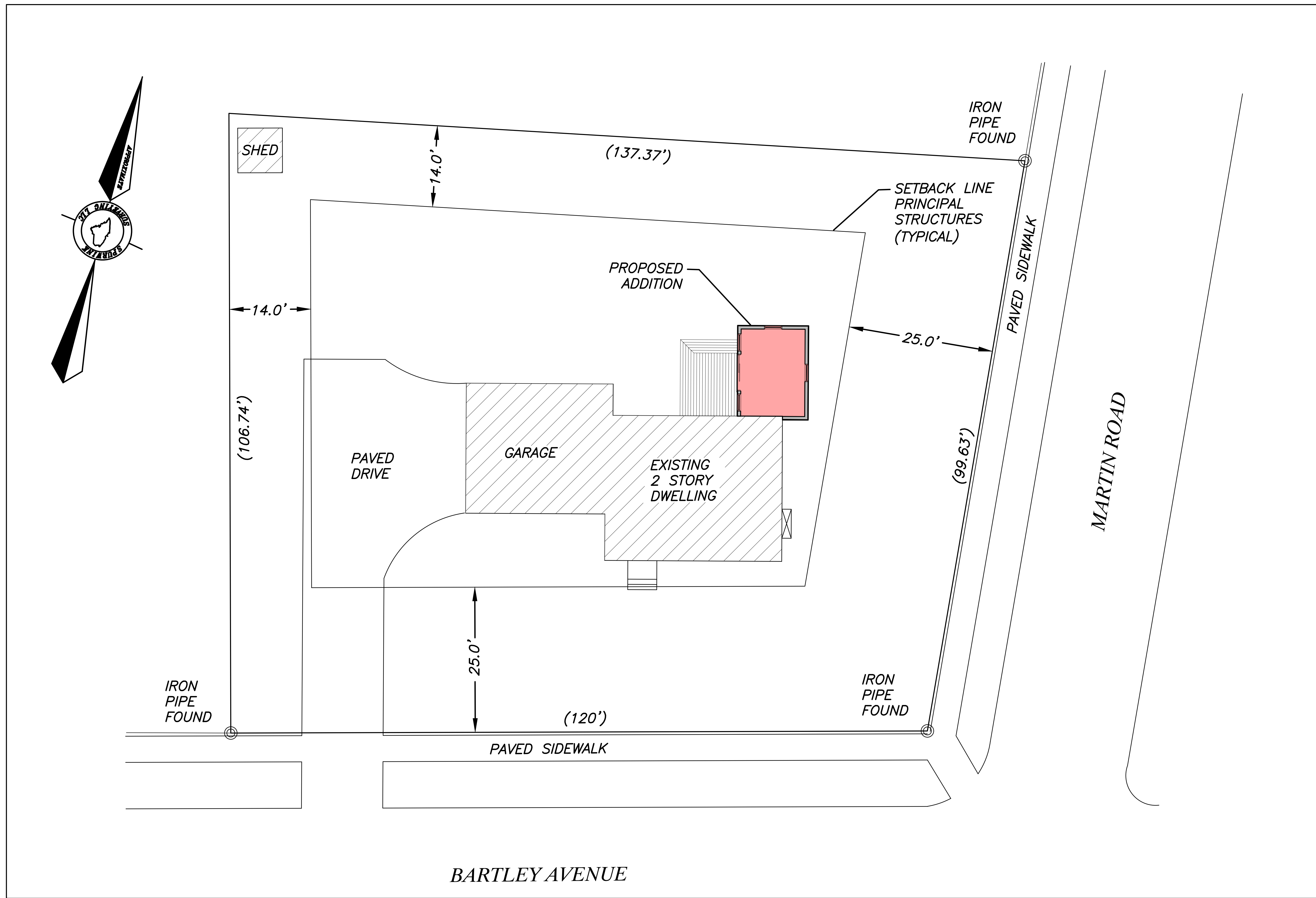
1 SITE PLAN 1/8" = 1'-0"
