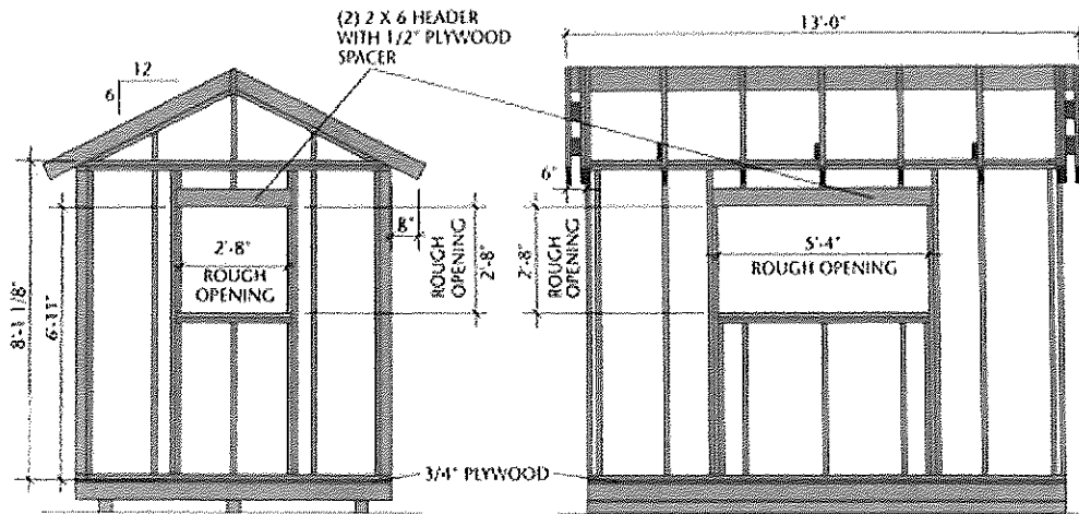
BUILDING SECTION
