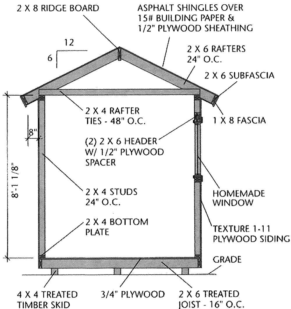
BUILDING SECTION
