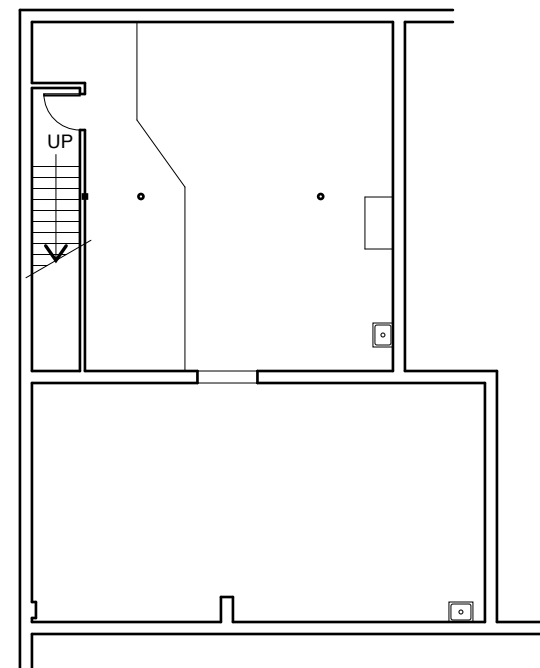
2 BASEMENT FLOOR PLAN SCALE: 1/16" = 1'-0" 4' 8' 16' 32'
