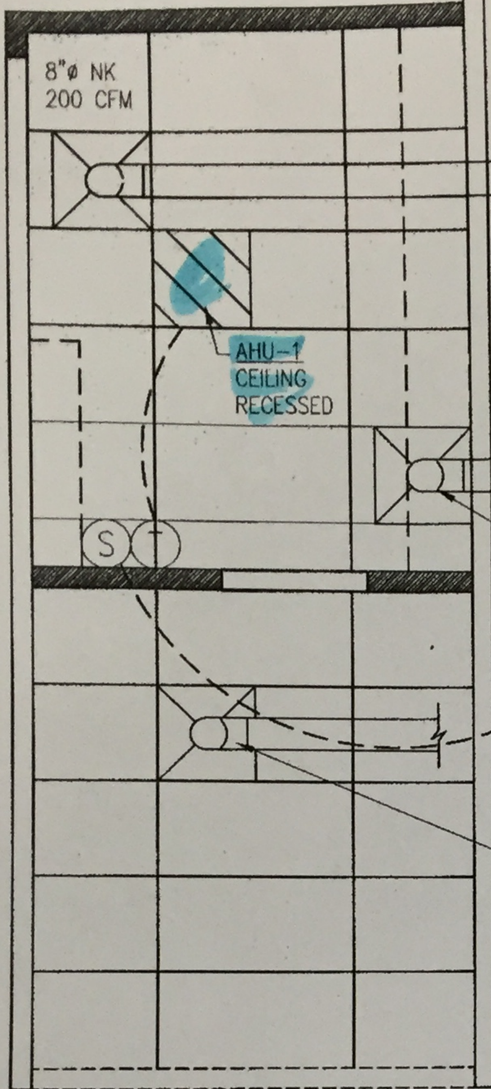
2 MINUTE CLINIC MECHANICAL PLAN A-3 SCALE: 1/4" = 1'-0"
