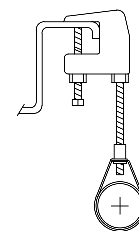
HANGER DETAIL TOP BEAM CLAMP
