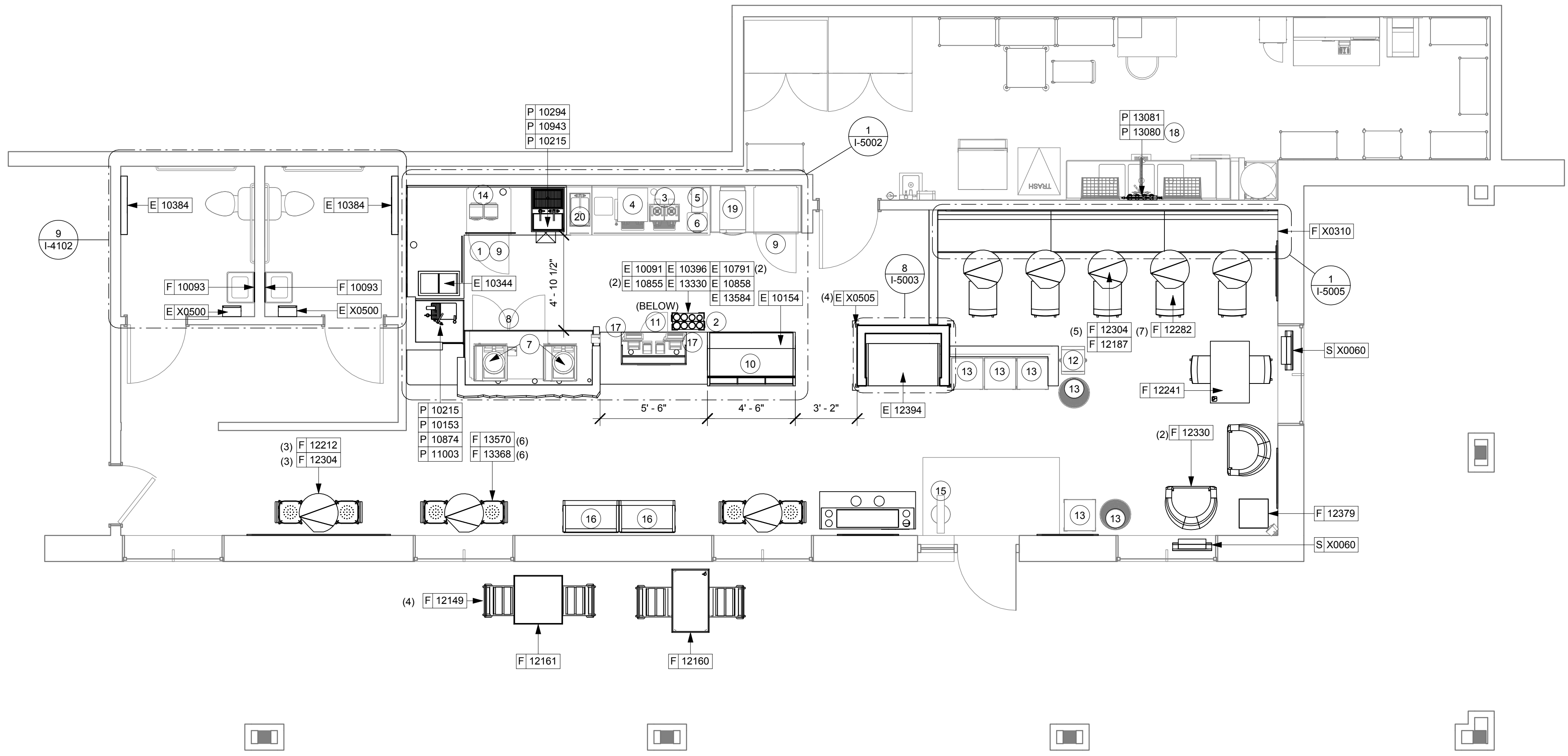
1ST FLOOR - FURNITURE, FIXTURES, AND EQUIPMENT PLAN Scale: 1/4" = 1'-0"
