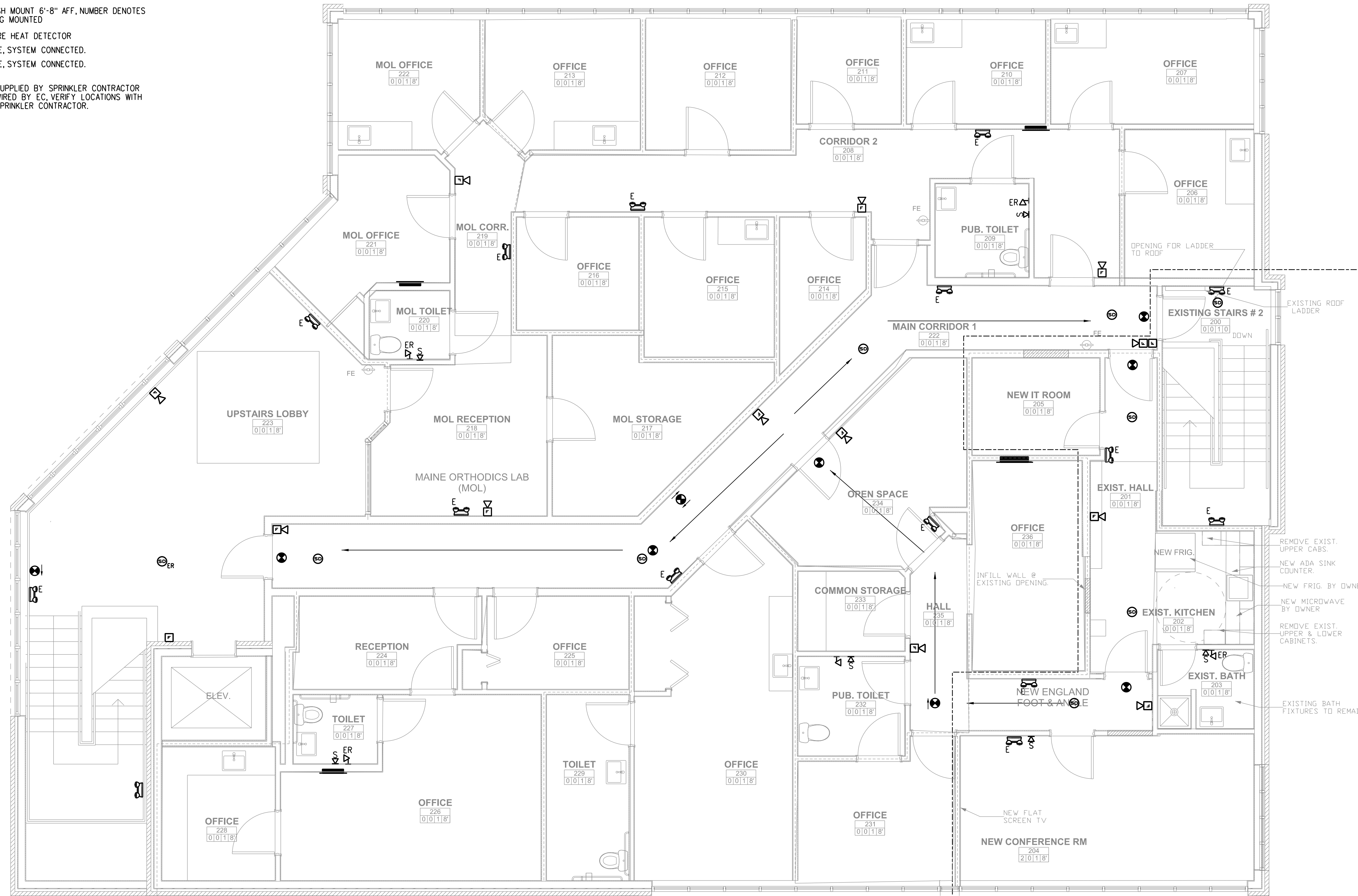
1 SECOND FLOOR LIFE SAFETY PLAN E2.2 SCALE: 1/4" = 1'-0"
