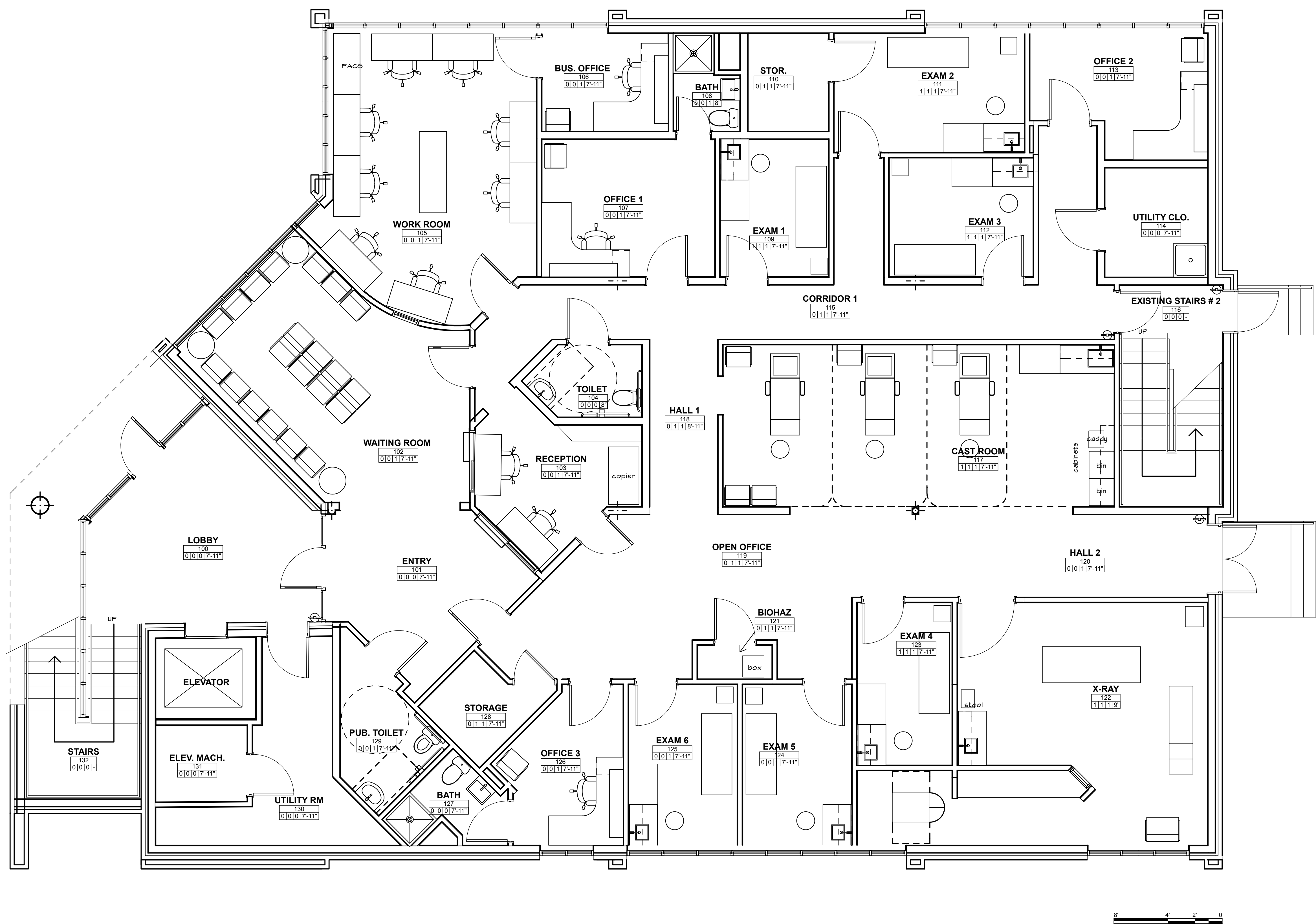
1 FIRST FLOOR FURNITURE PLAN SCALE: 1/4" = 1'-0"
