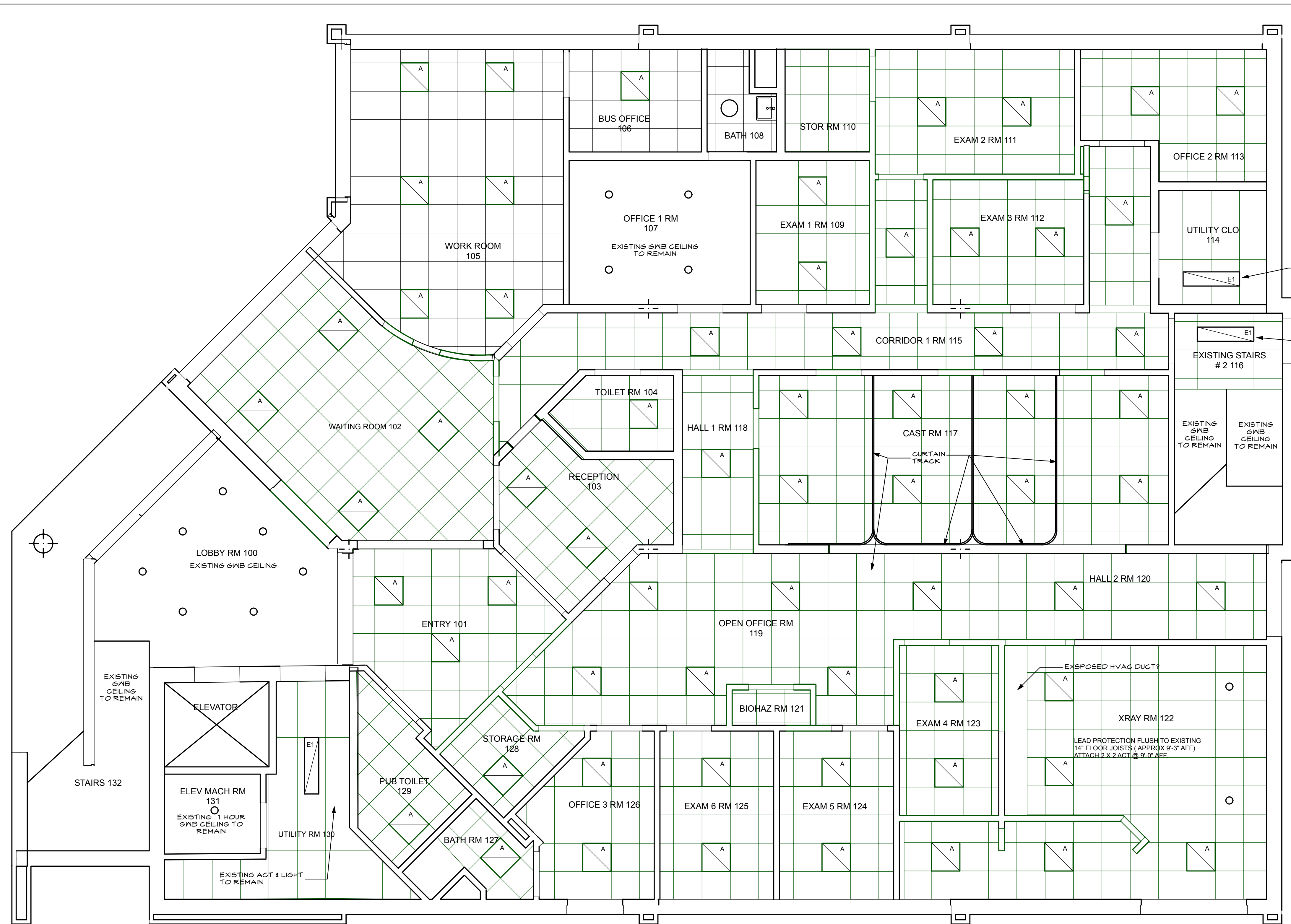
1 A1.4 FIRST FLOOR REFLECTED CEILING PLAN SCALE: 1/4" = 1'-0"
