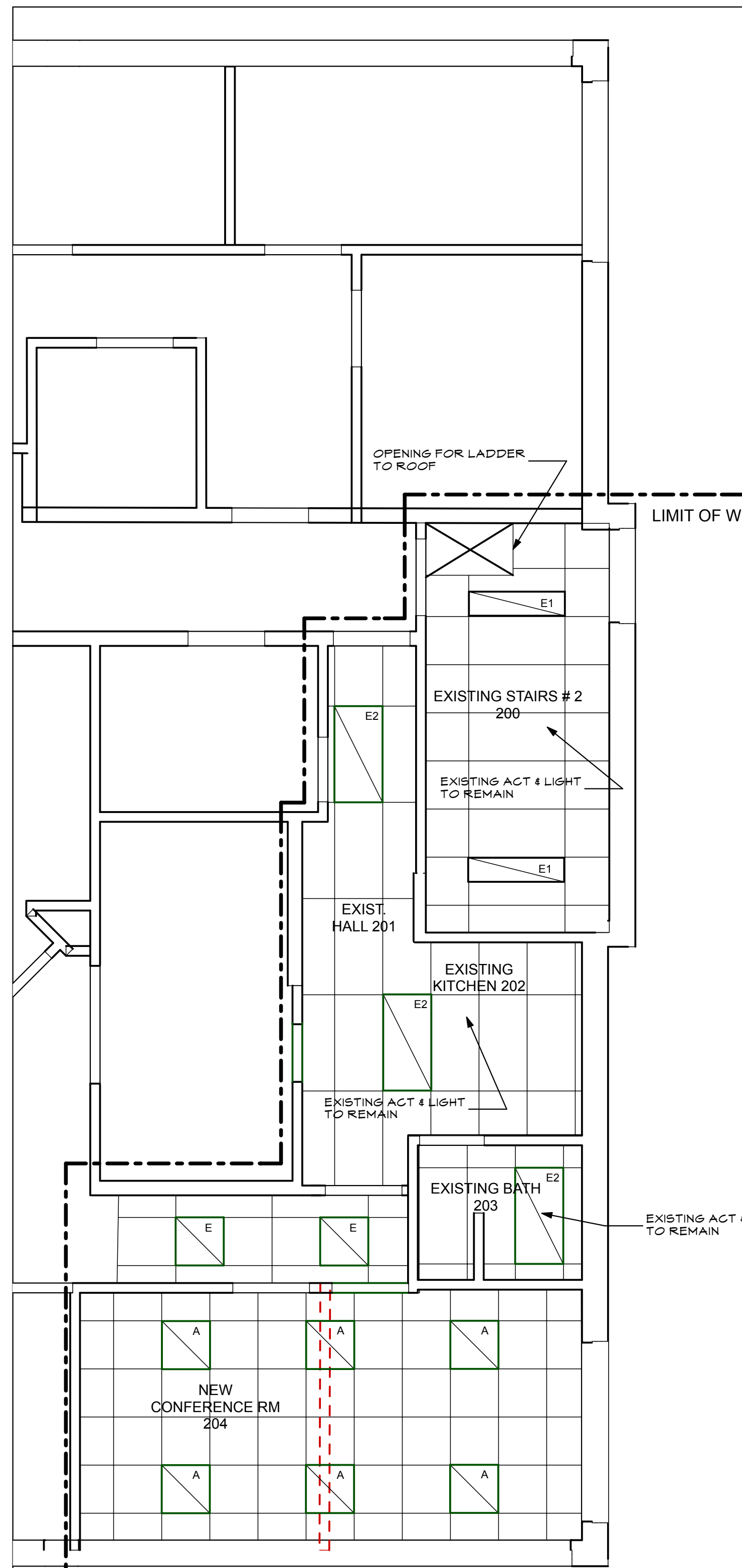
2 A1.4 IT OF WORK SECOND FLOOR RCP SCALE: 1/4" = 1'-0"
