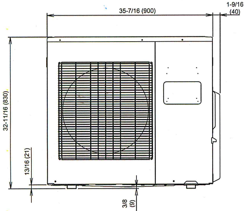
Front view
