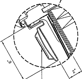
VELUX EDL Sill Flashing
