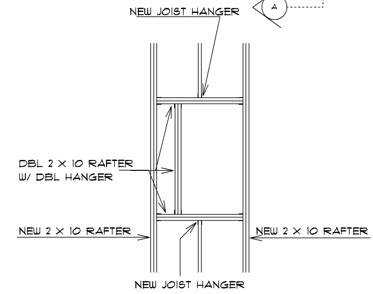
SKYLITE FRAMING DETAIL
