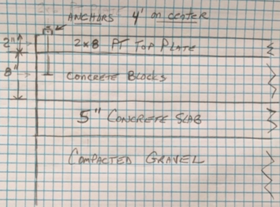
ELEVATION VIEW OF FOUNDATION
