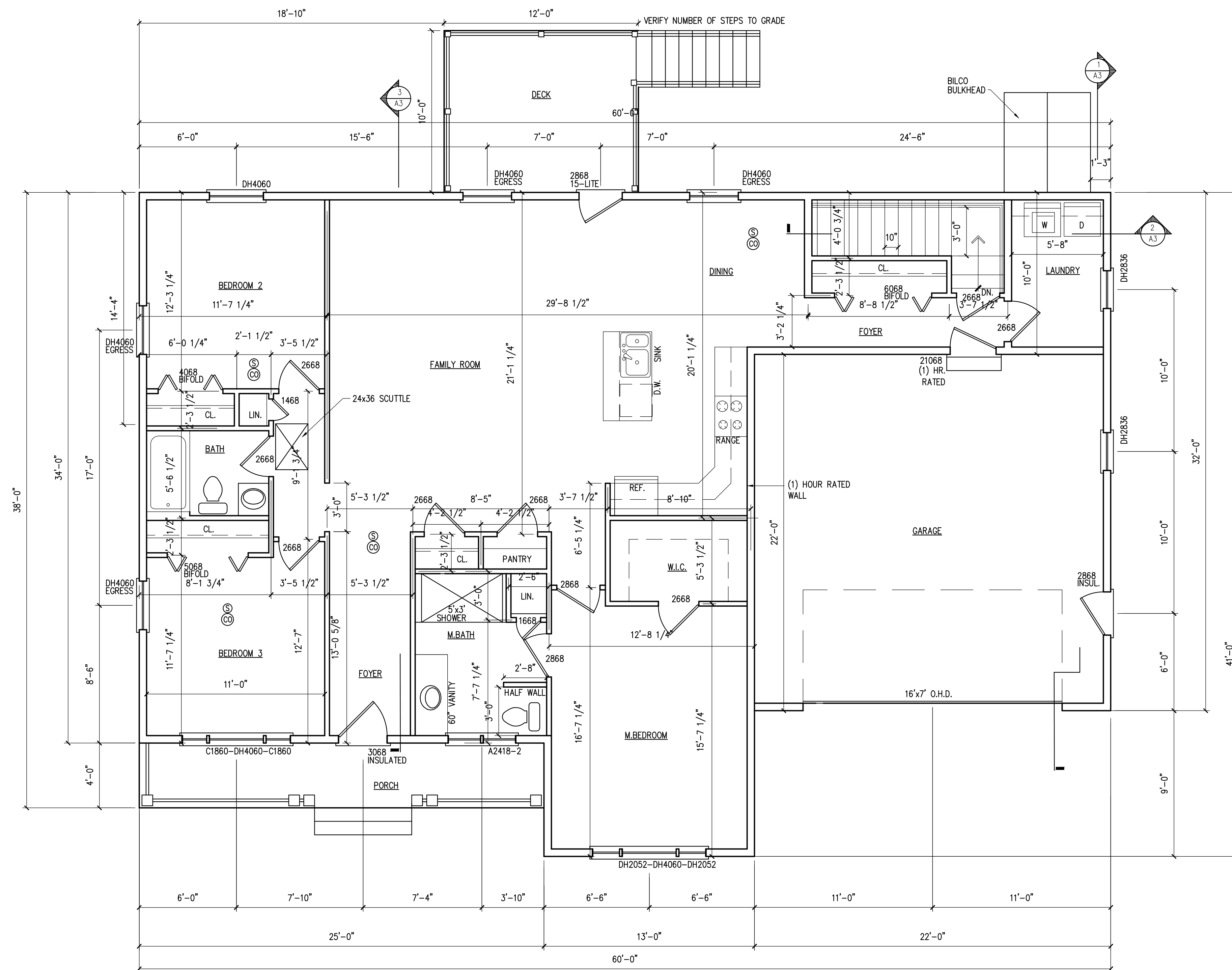
FIRST FLOOR HOUSE: 1,596 S.F. 1/4" = 1'-0" GARAGE: 550 S.F.
