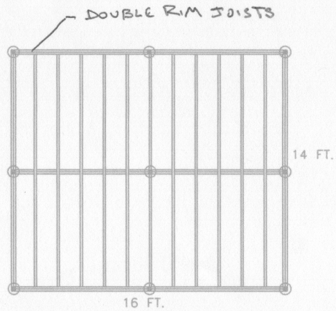
FLOOR JOIST W/CONCRETE PIERS
