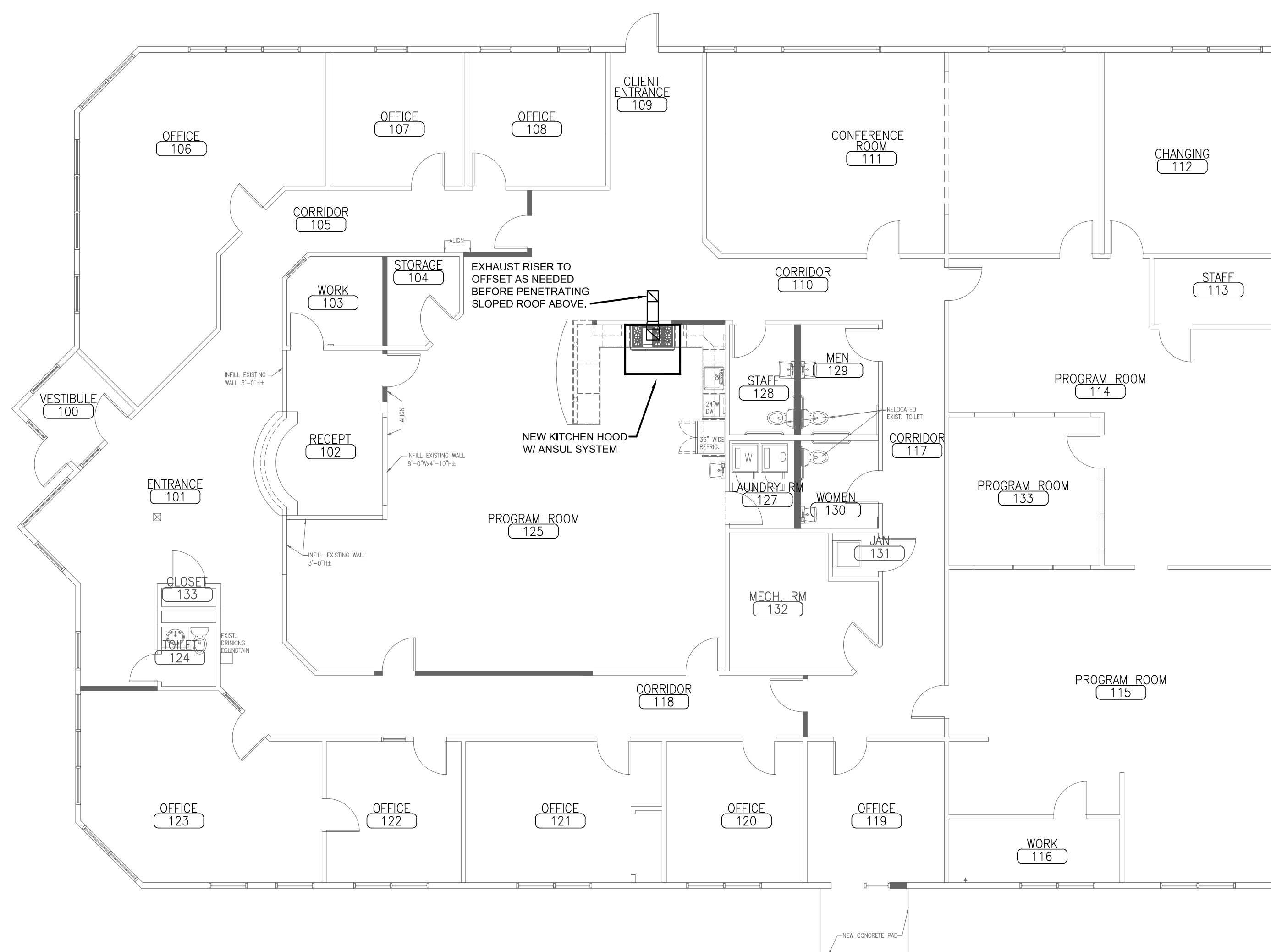
1 MECHANICAL HVAC - EXHAUST FAN & HOOD DUCTWORK PLAN SCALE: 1/8" = 1'-0"
