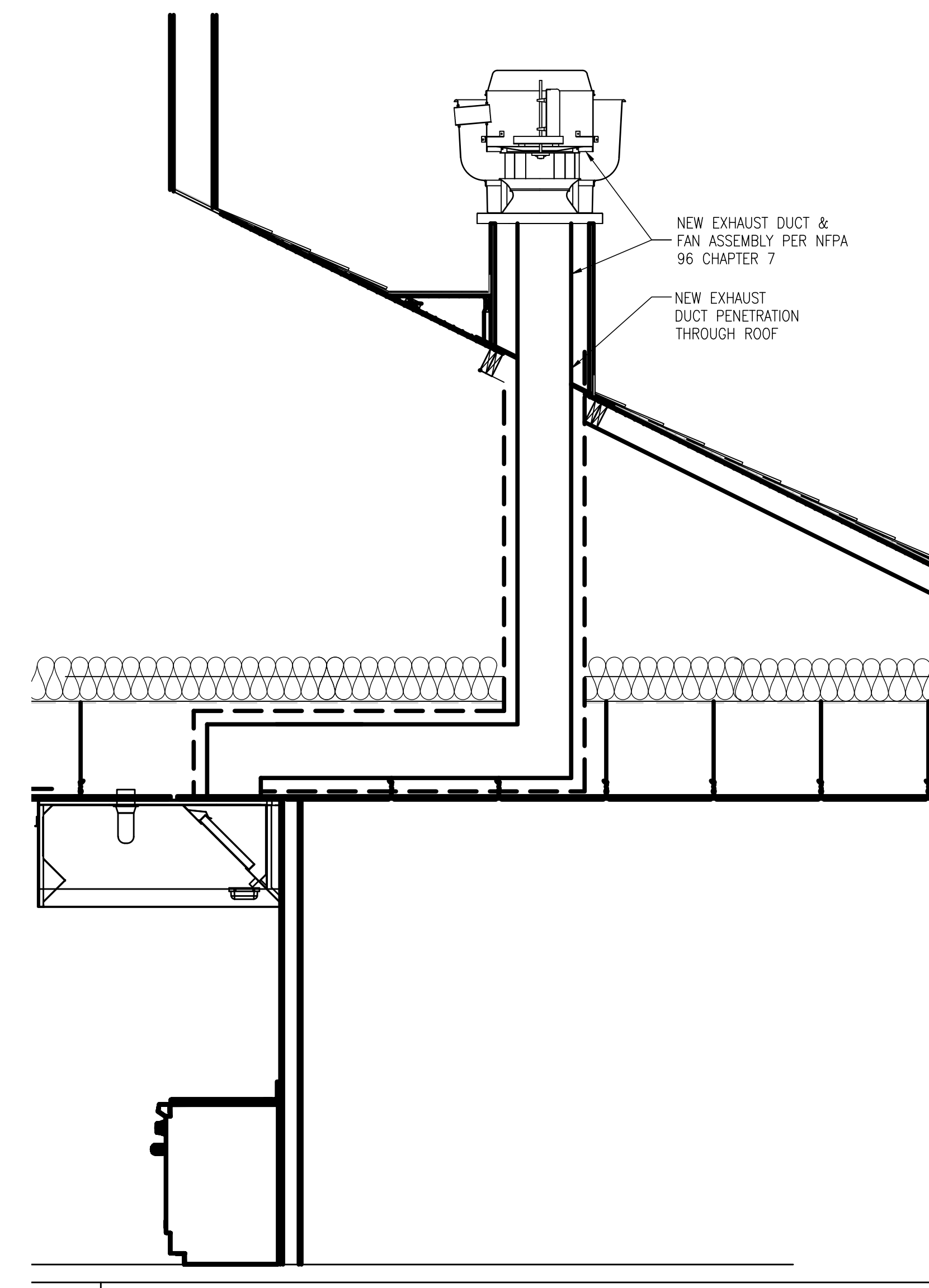
1 MECHANICAL HVAC - EXHAUST FAN & HOOD DETAIL SCALE: 1/2" = 1'-0"
