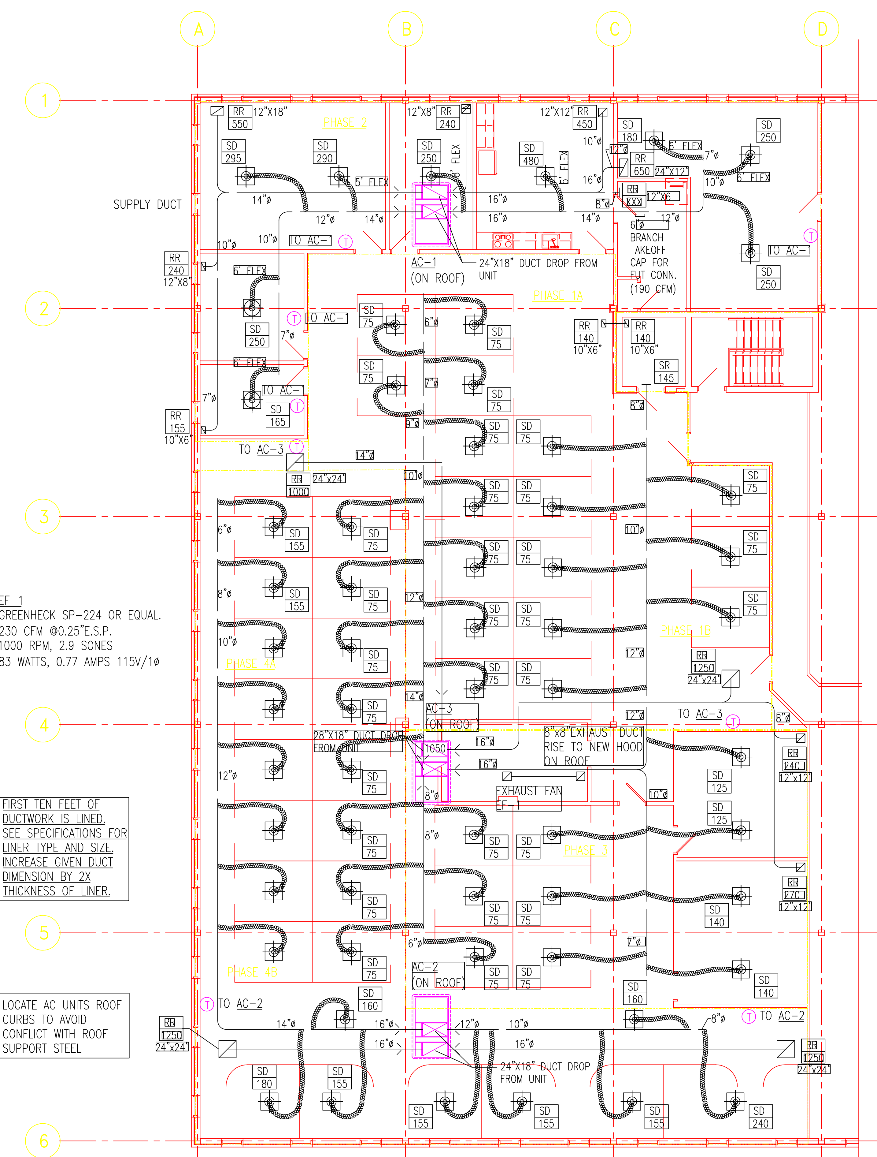
Renovated Floor Plan - Partial Plan Scale: 3/32" = 1'-0"
