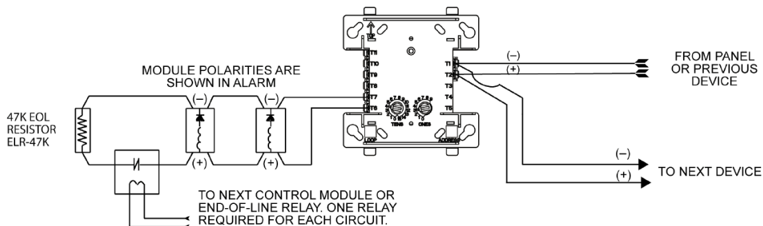
Notification Appliance Circuit NFPA Style Y
