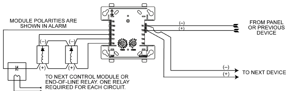
Notification Appliance Circuit NFPA Style Z
