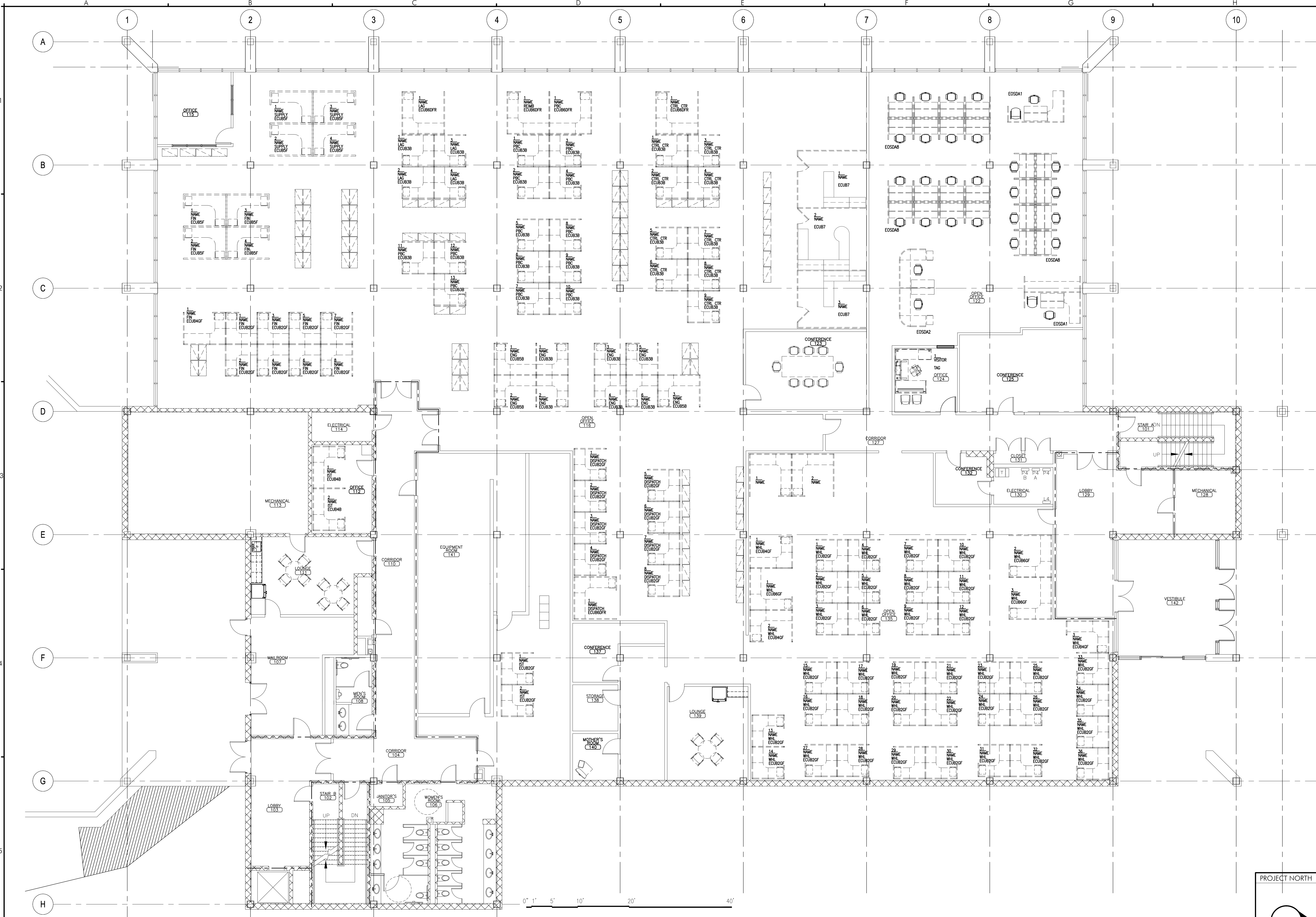
A5 FIRST FLOOR FURNITURE PLAN REFERENCED FROM: SCALE: 1/8" = 1'-0"
