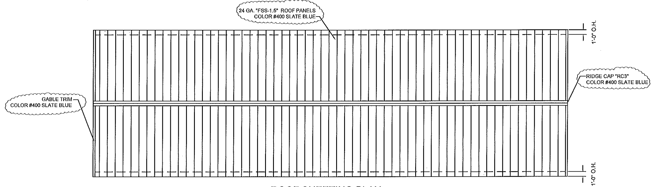
ROOF SHEETING PLAN
