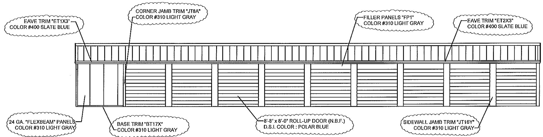
NEAR SIDEWALL ELEVATION
